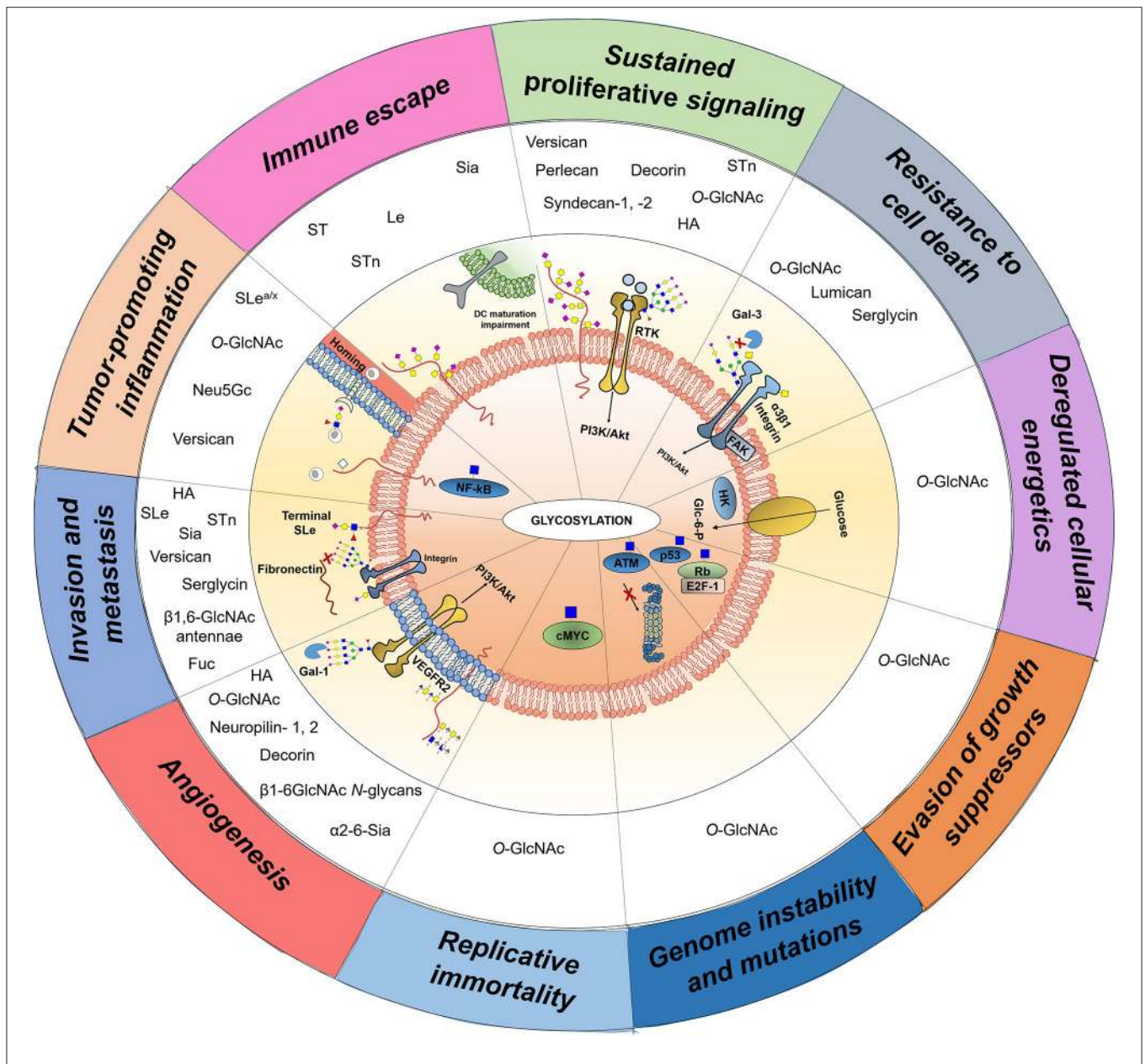
FIGURE 4 | Transversal nature of glycans, glycoproteins, glycan-binding proteins, and proteoglycans throughout the 10 currently accepted cancer hallmarks. Aberrantly expressed glycans (O-GlcNAc, Le, SLe a/x , Neu5Gc, Sialic acids (Sia), fucose residues (Fuc), ST, STn), glycoproteins (integrin α3β1, VEGFR2), and proteoglycans (Perlecan, Decorin, Neuropilin-1,-2, Syndecan-1,-2, Hyaluronic acid fragments (HA), Versican, Lumican, Serglycin) are mechanically involved in cancer hallmarks acquisition. The illustration highlights the most common glycosylation modifications throughout the cancer hallmarks, transmitting the empiric notion that a great number of glycosylation aberrations mostly contribute to disease dissemination through increased angiogenesis and potentiation of invasion and metastasis. Moreover, the post-translational modification β-O-N-acetyl-d-glucosamine (O-GlcNAc) emerges as a key regulator of cellular activities through the modulation of signal transduction and protein stabilization. In conclusion, glycans and glycoconjugates are not bystanders to malignant transformation but major players, making them attractive targets to drive molecular-based clinical intervention.
