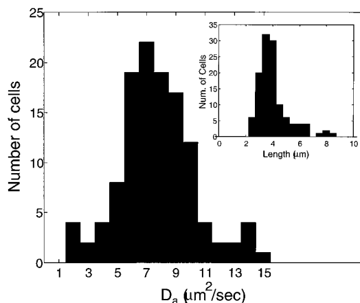
FIG. 3. Histogram of apparent diffusion coefficients for 120 DH5 \alpha cells measured by photobleaching. (Inset) Distribution of cell lengths for the same data. There is no significant correlation between cell length and apparent diffusion coefficient.
