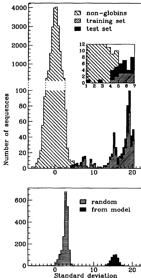
Figure 4: Histograms of the distance to the model measured in standard deviations from the average distance to the model for non-globins (see text).
