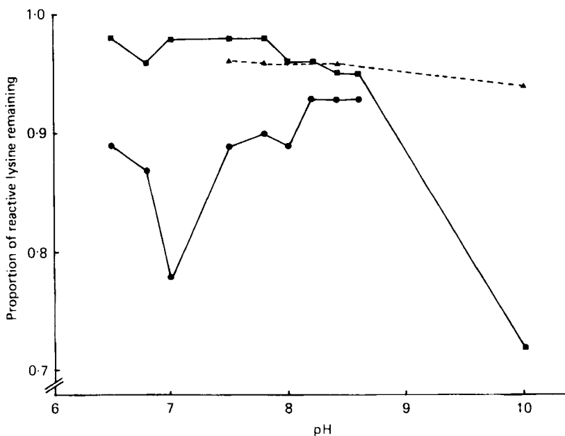
Fig. 1. Proportion of FDNB-reactive lysine remaining in casein-caffeic acid systems reacted at different levels of pH. (●), with tyrosinase ( EC 1.14.18.1); (■), without tyrosinase; (▲), without tyrosinase, without agitation, without oxygenation. Each value is the mean of duplicate determinations. The pooled SEM was 1.0 mg/g crude protein (nitrogen \times 6.25) corresponding to 0.012 on the proportion scale; the FDNB-reactive lysine content of the untreated casein was 82.0 mg/g crude protein. For experimental details, see p. 192.
