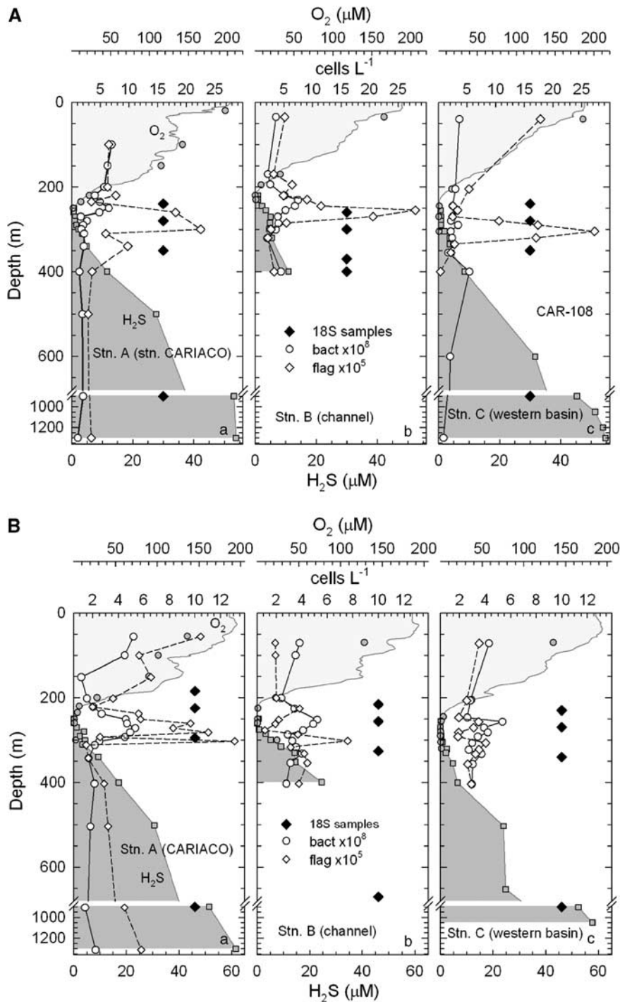
Figure 2 Vertical profiles of oxygen, hydrogen sulfide and bacterial and flagellate abundances at the time of sampling for protistan DNA in (A) January and (B) May 2005; modified from Taylor et al. (2001) and Scranton et al. (2006).
