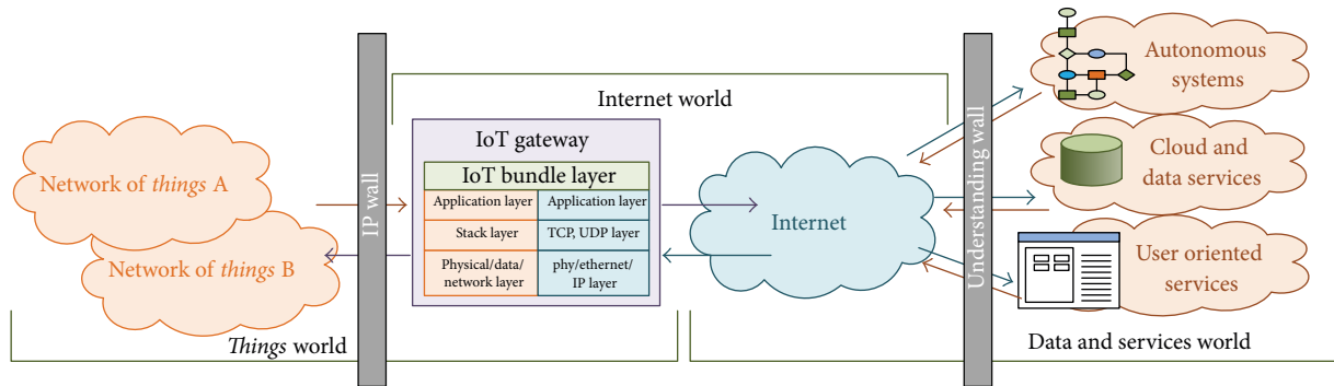
FIGURE 1: IoT architecture.
