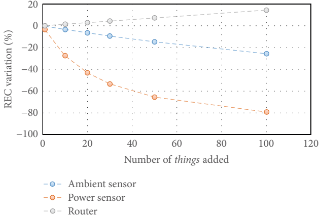
FIGURE 10: Relative energetic cost variation with respect to the proposed scenario when including new devices.
