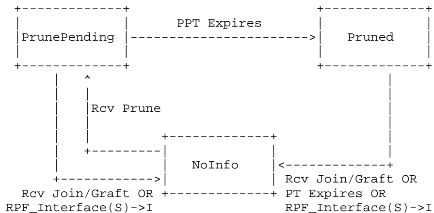
Figure 2: Downstream Interface State Machine
