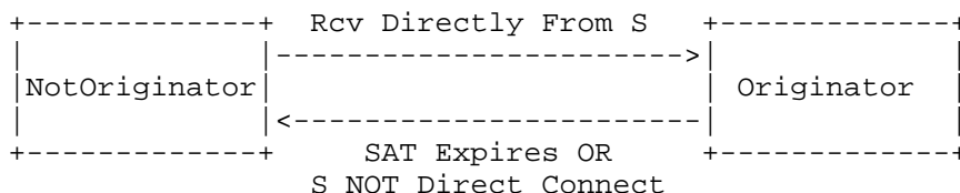
Figure 3: State Refresh State Machine
