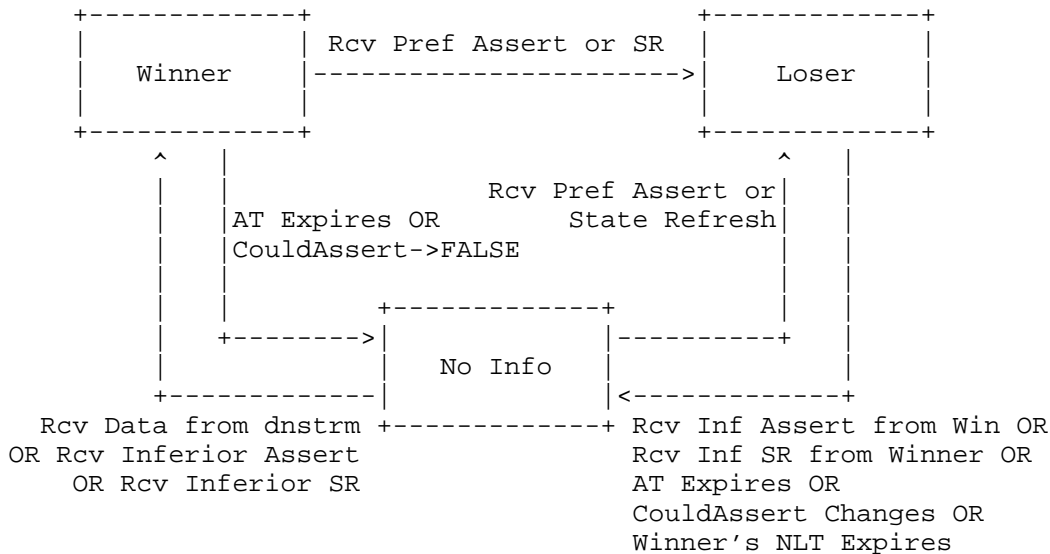
Figure 4: Assert State Machine
