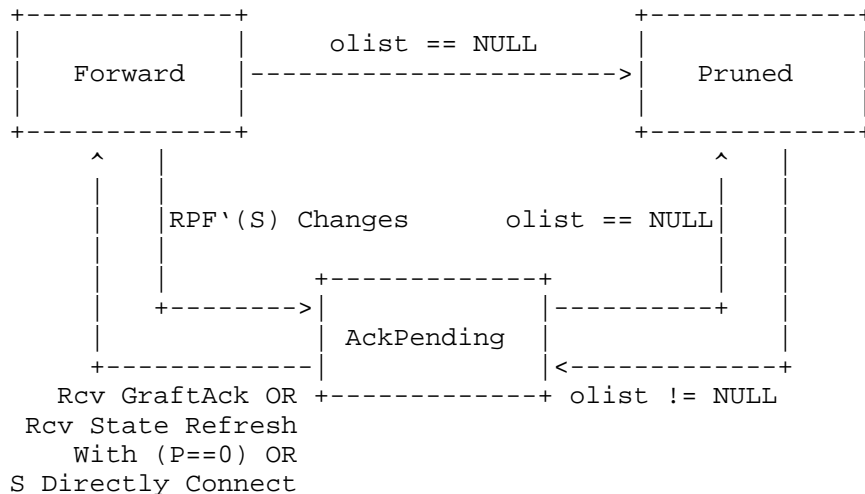
Figure 1: Upstream Interface State Machine
