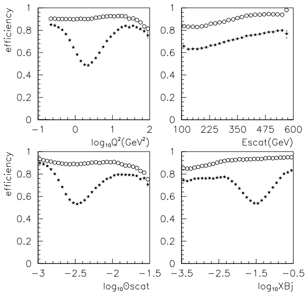
FIG. 17. Muon reconstruction efficiency predicted by the Monte Carlo. The curves in solid stars show the efficiency including the DC-PSA acceptance.
