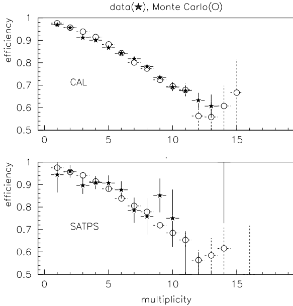
FIG. 11. Charged multiplicity dependence of the muon reconstruction efficiency measured from the data, compared with the prediction of the final tuned Monte Carlo. CAL and SATPS trigger samples are shown here.
