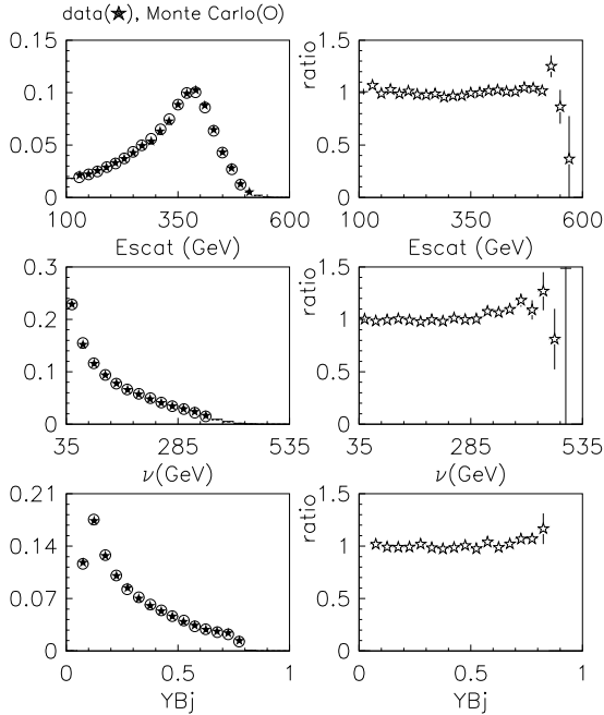
FIG. 33. (left) Final data-Monte Carlo comparisons of inclusive distributions. The distributions are normalized to integrate to unity before the comparison. (right) The ratio (data/MC) of the normalized data and Monte Carlo distributions. E_{scat} is the scattered muon energy, the other variables have their usual meaning.
