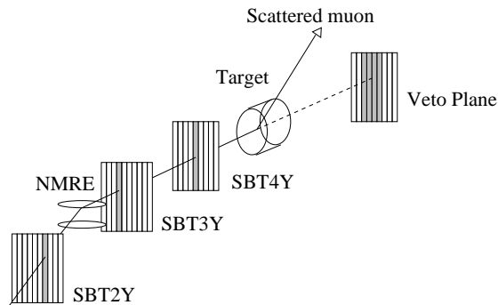
FIG. 2. Schematic diagram of the SAT.
