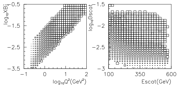
FIG. 25. SAT efficiency vs kinematic variables, predicted by Monte Carlo. The minimum efficiency shown is zero and the maximum is unity.
