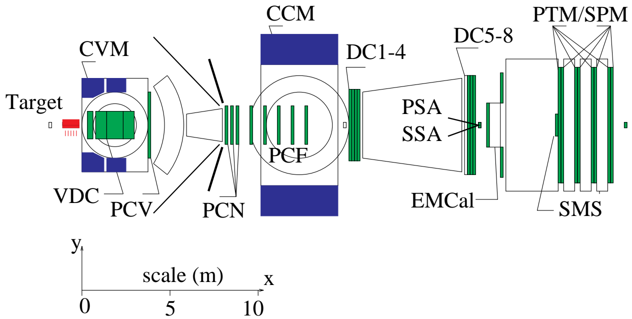
FIG. 1. The E665 forward spectrometer and muon detector.
