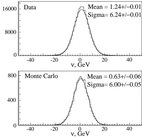
FIG. 27. Difference ( \nu ) between momenta of non-interacting beams as measured by the beam and forward spectrometers. The upper plot is obtained from the data and the lower from the Monte Carlo simulation. The curves are Gaussian fits to the distributions, with the parameters as indicated.
