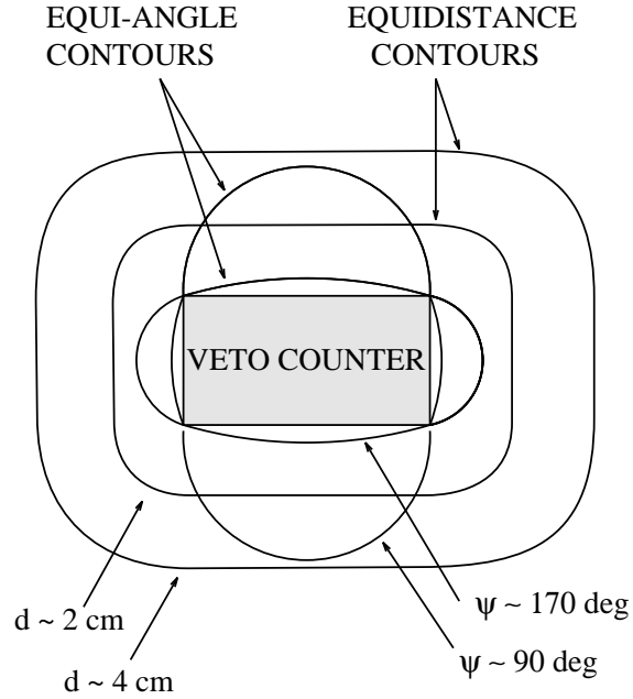
FIG. 20. Contours of equal d and \psi , which are the distance from the hodoscope and the angle subtended by the hodoscope.
