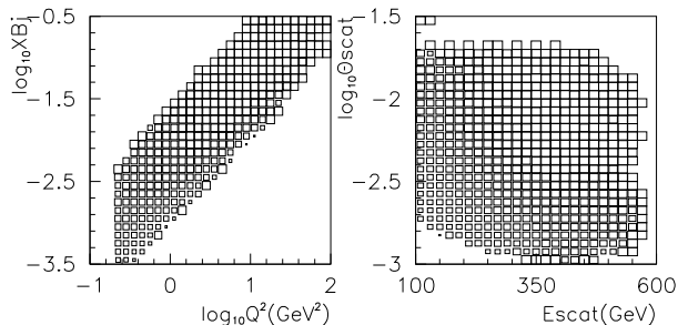
FIG. 26. SAT efficiency vs kinematic variables, predicted by Monte Carlo. A geometrical cut has been made around the SMS and SSA edges on the underlying muon distribution before the efficiency is computed. The minimum efficiency shown is zero and the maximum is unity.
