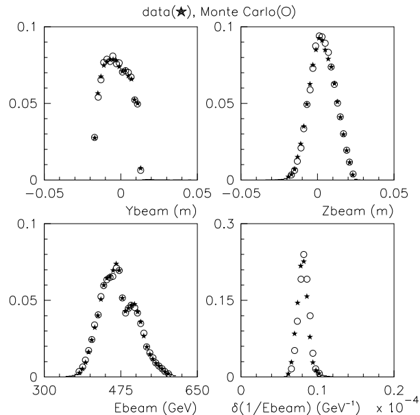
FIG. 32. Position and energy distributions of RSAT beam tracks, compared for Data and Monte Carlo.
