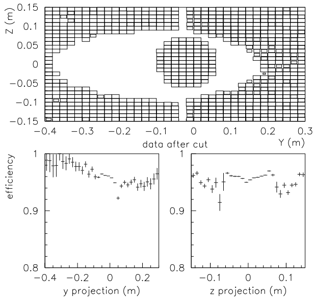
FIG. 14. DCA-DCB-PSA efficiency of contributing to the scattered muon track, measured from the data following cuts to eliminate dead regions. The efficiency is plotted vs the track coordinate at DCB
