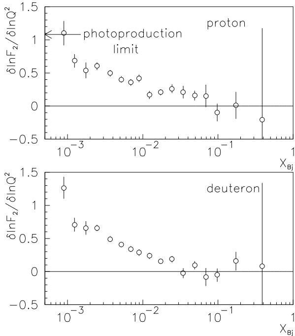
FIG. 44. Logarithmic derivative of F_2 with respect to Q^2 ( \partial \ln F_2 / \partial \ln Q^2 ) at fixed x , shown vs x for proton and deuteron. The photoproduction limit [18] derived from real photon-proton cross-section measurements is also shown.
