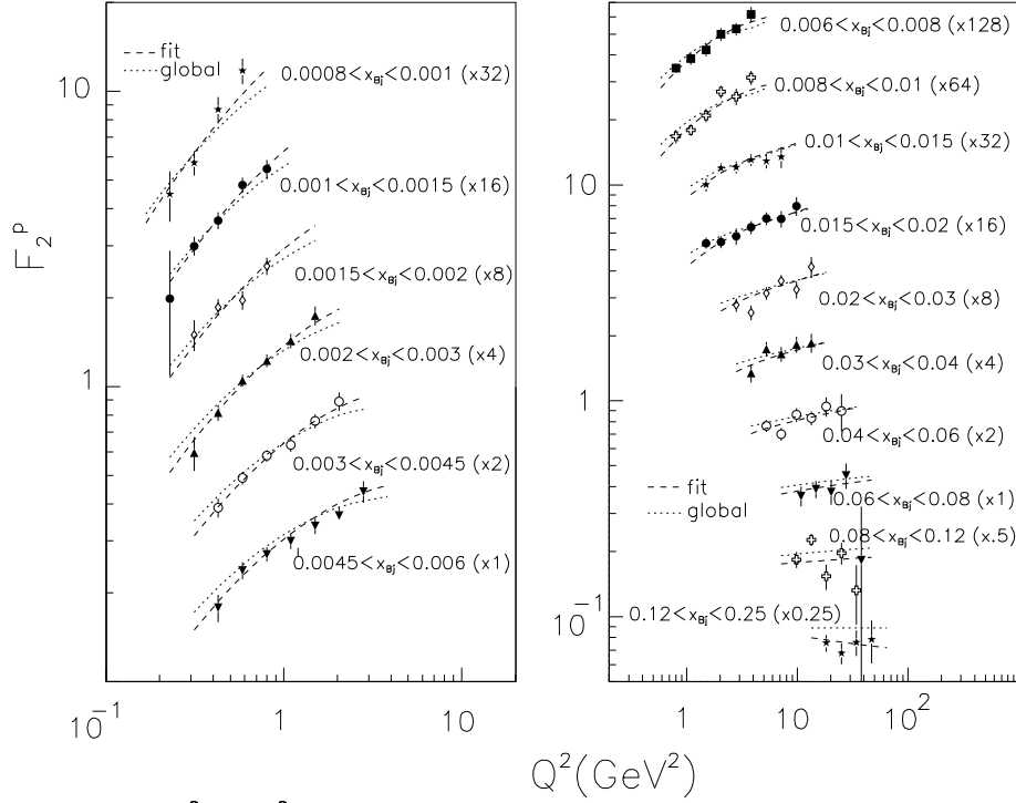
FIG. 40. proton F_2 vs Q^2 ( \text{GeV}^2 ) in x_{Bj} bins, with curves showing the fit to the data and the global F_2 parametrization [41].
