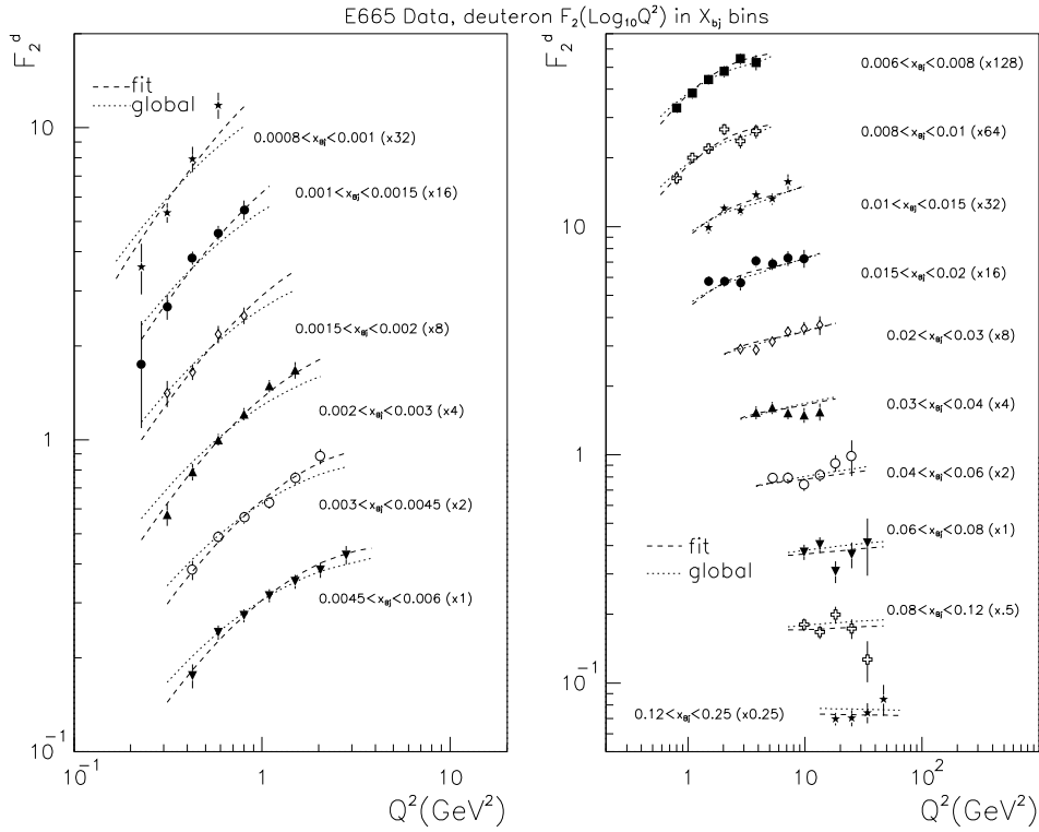
FIG. 41. deuteron F_2 vs Q^2 ( \text{GeV}^2 ) in x_{Bj} bins, with curves showing the fit to the data and the global F_2 parametrization.
