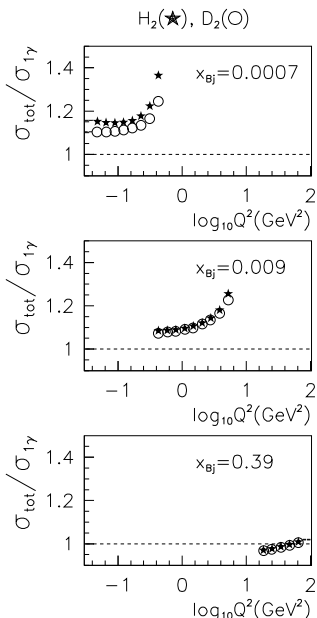
FIG. 31. Calculated radiative correction \sigma_{tot}/\sigma_{1\gamma} for proton and deuteron, shown as a function of \log_{10}(Q^2/\text{GeV}^2) in bins of x_{Bj} .
