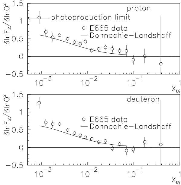
FIG. 55. Logarithmic derivative of F_2 with respect to Q^2 at fixed x , shown vs x for proton and deuteron. The photoproduction limit [18] derived from real photon-proton cross-section measurements is also shown. The data are compared with the Donnachie-Landshoff model.
