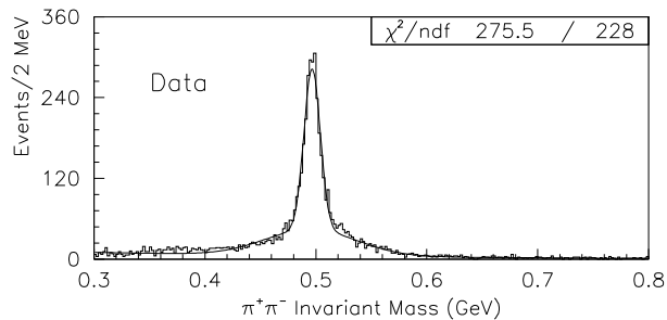
FIG. 29. The \pi\pi invariant mass distribution for V^0 vertices that pass the K_s^0 selection. The curve is the sum of two Gaussians and a polynomial fitted to the data. The fitted mean of the narrow peak is (496.6 \pm 0.2) MeV and its r.m.s. is (7.4 \pm 0.3) MeV.
