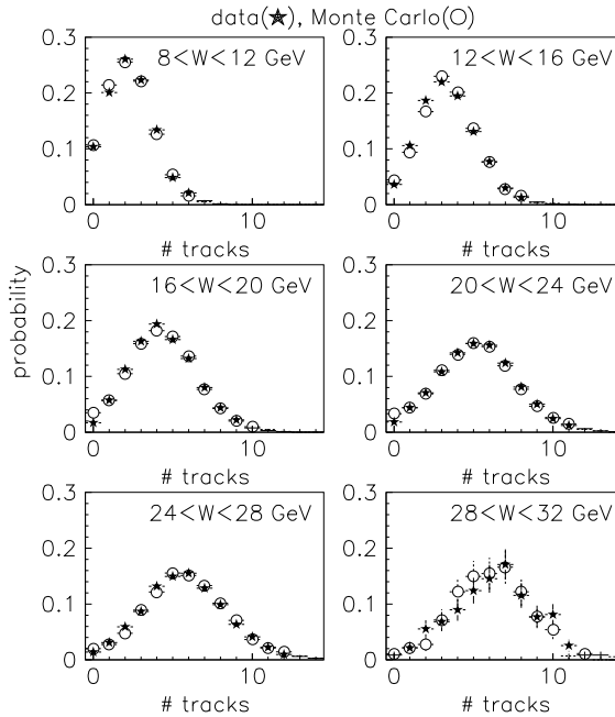
FIG. 9. Normalized multiplicity distributions in W bins, for Data and Monte Carlo. Each distribution has been normalized to integrate to unity. Hadronic scatters selected using the calorimeter are used. Only SATPS and SVS triggers are included. The multiplicity in the Monte Carlo simulation has been multiplied by 1.08, giving a good match with the data.
