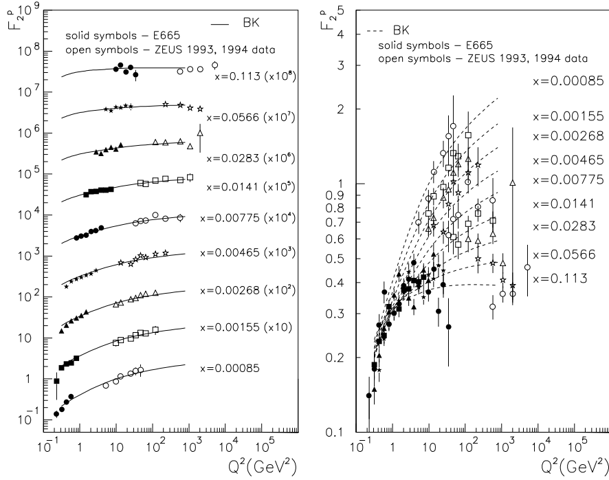
FIG. 49. proton F_2 vs Q^2 (GeV 2 ) in x_{Bj} bins, from E665 and ZEUS [67]. The Badełek-Kwieciński (BK) model is also shown. (left) The data points and the model curves have been multiplied by the factors indicated in parentheses for clarity. (right) The points and curves are plotted with no scale factors, to show the trends.
