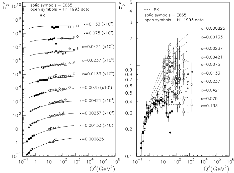
FIG. 50. proton F_2 vs Q^2 (GeV 2 ) in x_{Bj} bins, from E665 and H1 [68]. The Badełek-Kwieciński (BK) model is also shown. (left) The data points and the model curves have been multiplied by the factors indicated in parentheses for clarity. (right) The points and curves are plotted with no scale factors, to show the trends.
