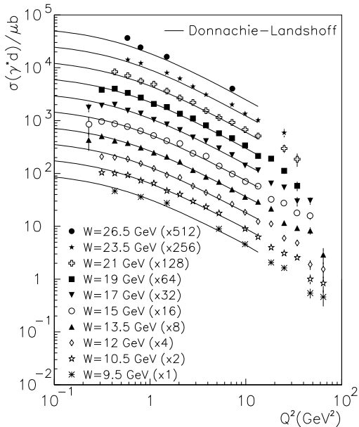
FIG. 57. Q^2 dependence of the virtual photoabsorption cross section for deuteron in W bins, compared with the Donnachie-Landshoff model.
