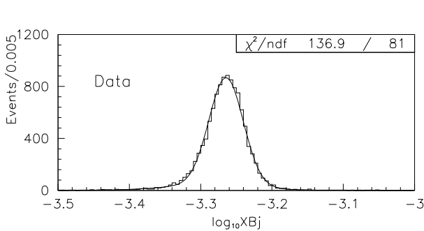
FIG. 28. \log_{10}x_{Bj} for data events passing the \mu e selection. The curve is a sum of two Gaussians fitted to the data. The mean of the main peak is -3.2643 \pm 0.0003 and the r.m.s. is 0.0241 \pm 0.0003 .
