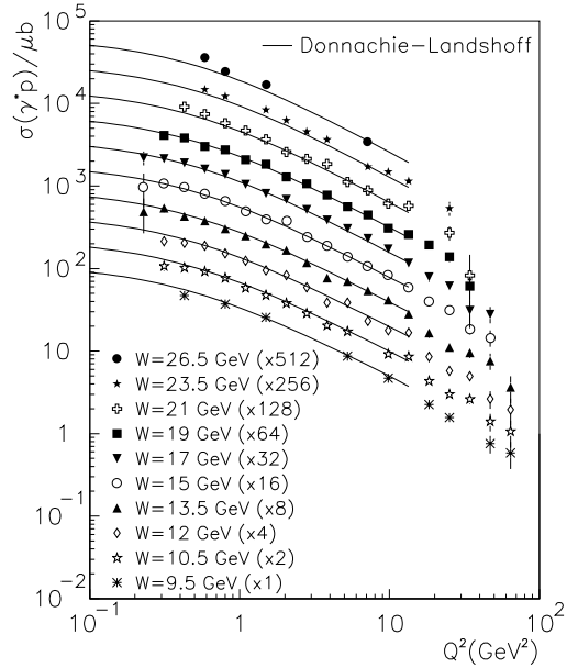
FIG. 56. Q^2 dependence of the virtual photoabsorption cross section for proton in W bins, compared with the Donnachie-Landshoff model.
