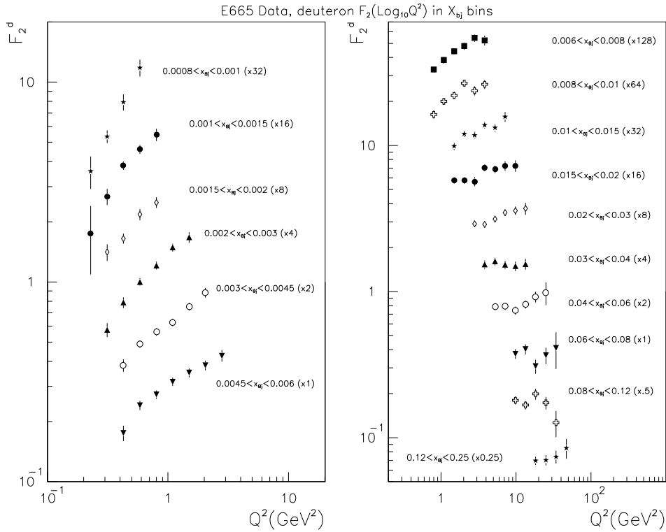
FIG. 37. deuteron F_2 vs Q^2 (GeV 2 ) in x_{Bj} bins.
