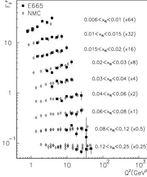
FIG. 47. proton F_2 from E665 and NMC [66] over-plotted vs Q^2 in x bins. In certain x bins one of the two experiments has multiple data points because the actual binning in x is narrower. In these cases all the data points falling in those bins are shown. The points have been multiplied by the factors indicated in parentheses for clarity.
