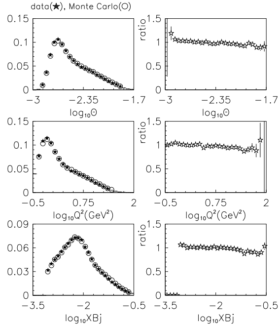
FIG. 34. (left) Final Data-Monte Carlo comparisons of inclusive distributions. The distributions are normalized to integrate to unity before the comparison. (right) The ratio (data/MC) of the normalized data and Monte Carlo distributions. \theta is the muon scattering angle in radians, the other variables have their usual meaning.
