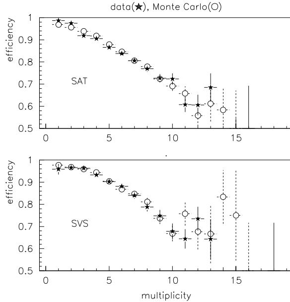
FIG. 12. Charged multiplicity dependence of the muon reconstruction efficiency measured from the data, compared with the prediction of the final tuned Monte Carlo. SAT and SVS trigger samples are shown here.
