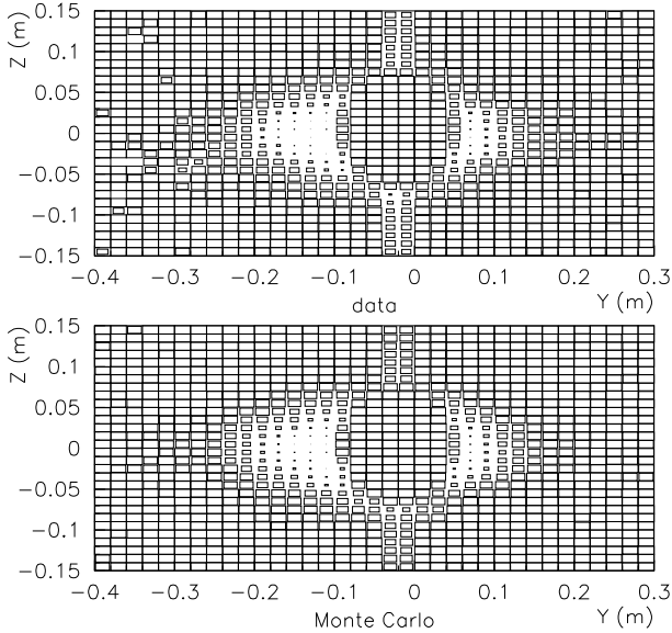
FIG. 13. DCA-DCB-PSA efficiency of contributing to the scattered muon track, measured from the Data (upper) and Monte Carlo simulation (lower) using PC-PCF tracks. The efficiency is plotted vs the track coordinates at DCB.
