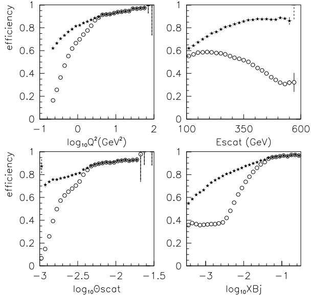
FIG. 24. SAT efficiency vs kinematic variables, predicted by Monte Carlo, shown using open circles. For the curves shown using solid stars, a geometrical cut has been made around the SMS and SSA edges on the underlying muon distribution before the efficiency is computed.
