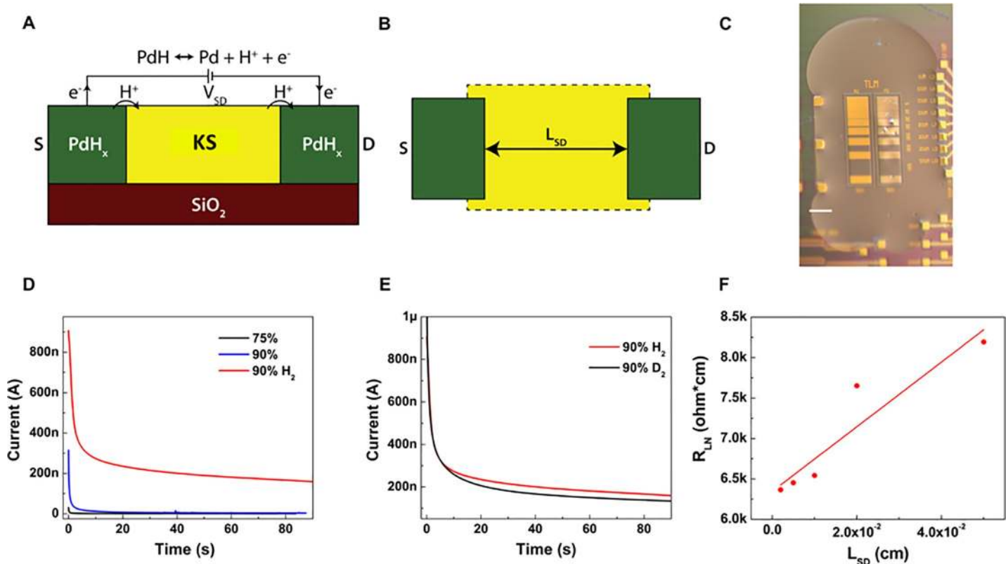
Fig 2. Proton conduction measurement of KS. A ) Palladium hydride(PdH x ) electrode behavior. Under a V SD , PdH x source split into Pd, H + , and e - . Protons are injected into the KS, whereas electrons travel through external circuitry and are measured. B ) TLM geometry. Varying the distance between source and drain (L SD ) distinguishes between the fixed PdH x -KS interface contact resistance and the varying bulk resistance. C ) Optical image of TLM geometry with hydrated KS on the surface. Scale bar, 500μm. D ) Transient response to a 1V bias in KS at 75%, 90%, 90% H 2 RH, in which the current under 90% with hydrogen is much higher than that under 90% RH without hydrogen. E ) Deuterium current (black) at 90% D 2 humidity is lower than proton current (red). F ) The normalized resistance R LN as a function of L SD . A linear fit gives a bulk material proton conductivity of 0.50 ± 0.11 mS cm -1 .
