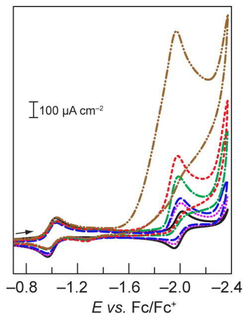
Figure S6. CVs of a 1.0 mM solution of 3 in the absence of benzoic acid (—) and in the presence of 0.5 (•••), 1.0 (— —), 3.0 (— •), 6.0 (— — —), and 20 mM (— ••) benzoic acid. Scan rate, 30 \text{ mV s}^{-1} ; 0.2 M TBAPF 6 in acetonitrile. Glassy carbon working electrode, Ag/AgNO 3 reference electrode, and Pt wire counter electrode.
