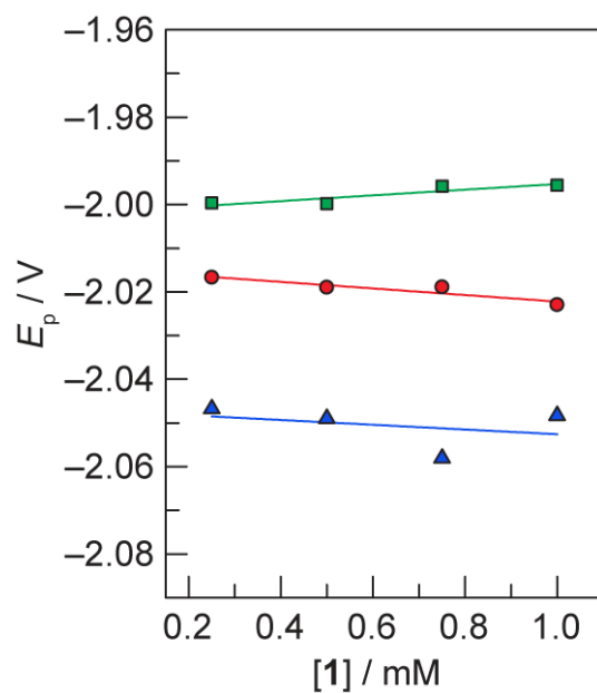
Figure S3. Concentration dependence studies of the Co^{+0} reduction wave peak potential of 1 . Experimental data obtained at scan rates of 0.03 (■), 0.3 (●), and 3 (▲) V s^{-1} .
