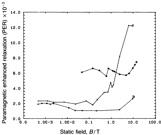
Fig. 5. The experimental complex-ligand proton PER of the complexes (a) \text{Ni}(\text{H}_2\text{O})_6^{2+} , (b) \text{Ni}(\text{dpm})_2\text{D}_5\text{NH}_2^{2+} and (c) \text{Ni}(\text{R},\text{S},\text{R},\text{S})1,2,8,11 -tetramethyl-1,2,8,11-tetraazacyclotetradecane)- (\text{H}_2\text{O})^{2+} (from Ref. 19).
