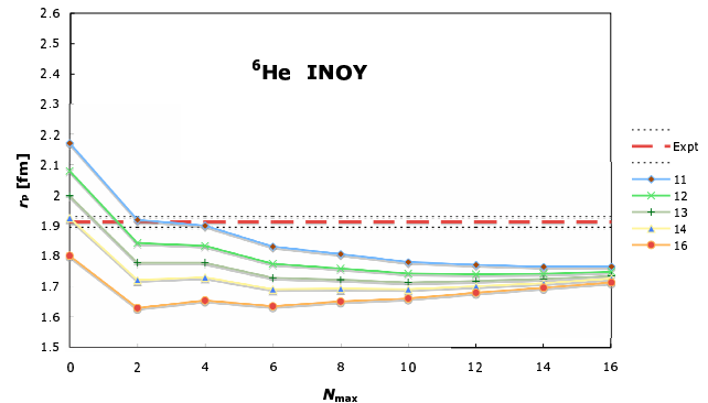
FIG. 7: The same as in Fig. 5, but for the INOY NN potential and HO frequencies from \hbar\Omega = 11 MeV to \hbar\Omega = 16 MeV.
