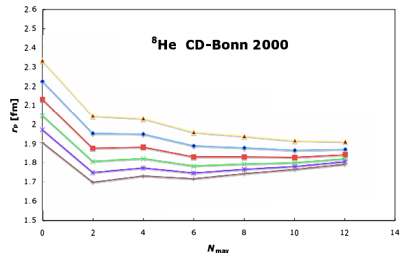
FIG. 8: The {}^8\text{He} point-proton rms radius dependence on the model space size for different HO frequencies from \hbar\Omega = 10 MeV to \hbar\Omega = 15 MeV obtained using the CD-Bonn 2000 NN potential.
