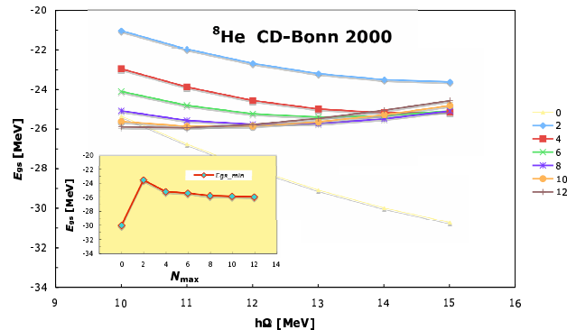
FIG. 3: The same as in Fig. 1, but for {}^8\text{He} and model-spaces from N_{\text{max}} = 0 to N_{\text{max}} = 12 .
