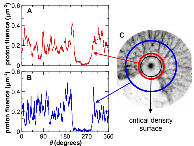
Fig. 5: Circular lineouts of proton fluence obtained from OMEGA shot 46529 at radii of 430 \mu\text{m} (A) and 860 \mu\text{m} (B). The filamentary structures represent a 2-dimensional (2-D) projection of a 3-D field structure that originates inside the critical density surface (C).
