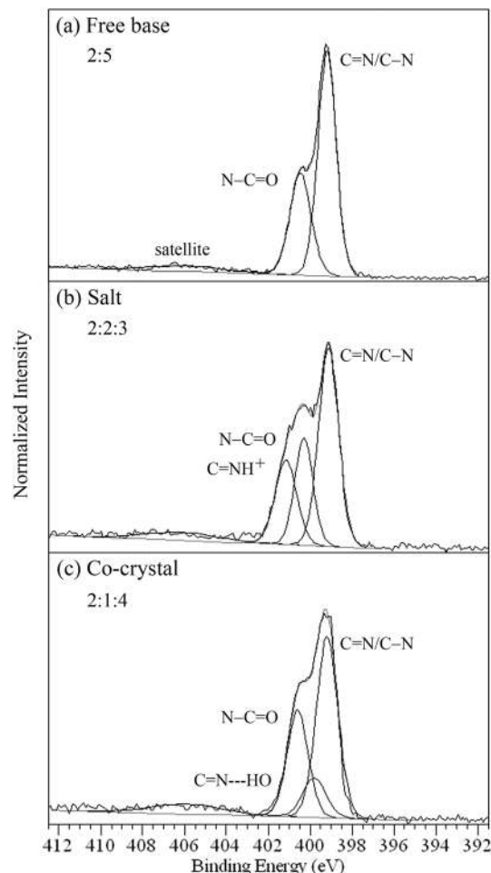
Fig. 5 N 1s XPS spectra of (a) the free base 1 , (b) di-HCl salt 1s , and (c) fumaric acid co-crystal 1c showing the ratios for the types of nitrogen.
