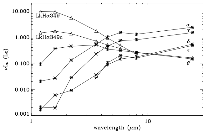
FIG. 4.—Spectral energy distributions for five newly discovered protostars ( \alpha – \epsilon ) and the two previously known young stars (LkH \alpha 349a and 349c). The spectrum of LkH \alpha 349a provides a reference for photospheric emission, while the others show varying degrees of infrared excess.
