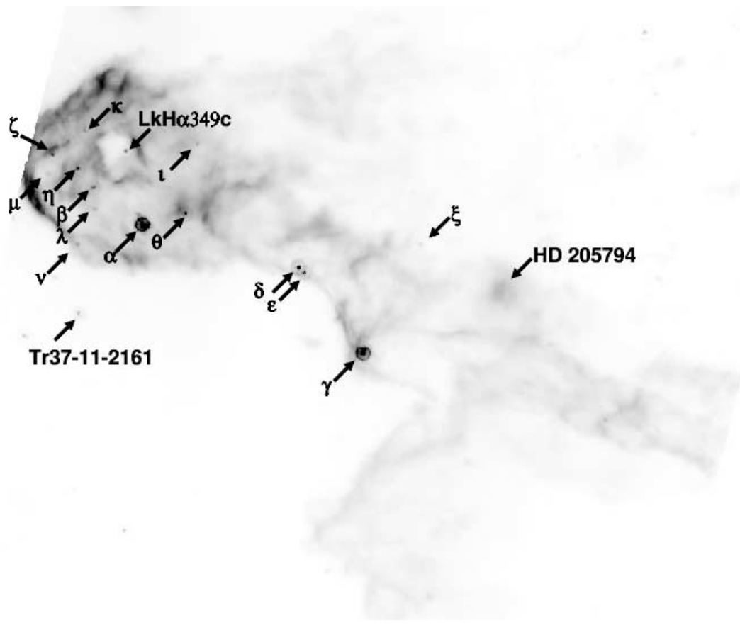
FIG. 2.— Spitzer /MIPS 24 \mu\text{m} image of the Elephant Trunk Nebula with newly discovered sources ( \alpha – \xi ) labeled. North is up, and east is to the left.
