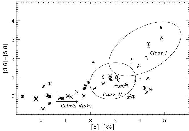
FIG. 3.— Spitzer color-color diagram for 24\ \mu\text{m} -detected sources in the Elephant Trunk Nebula (IC 1396A). Labeled points are from Table 1. The approximate locations of Class I and II protostars and main-sequence stars with debris disks are outlined.
