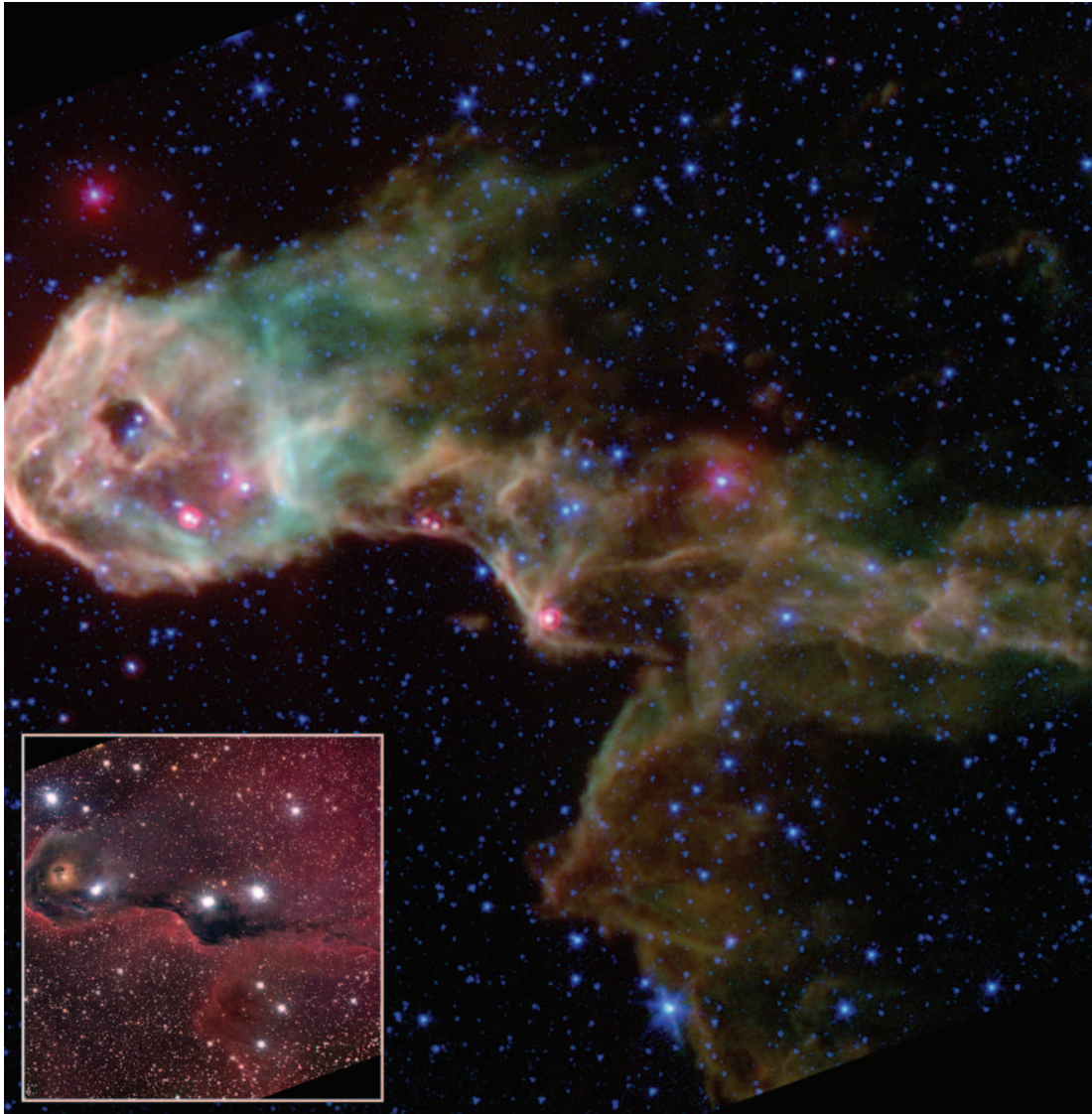
FIG. 1.— Spitzer image of the Elephant Trunk Nebula in IC 1396, combining the MIPS 24 \mu\text{m} ( red ) and IRAC 5.8+8 \mu\text{m} ( green ) and 3.6+4.5 ( blue ) \mu\text{m} images. The inset shows the optical image, combining red, green, and blue images from the CFHT. [This figure is available as an mpeg file in the online edition of the Journal .] The animation begins with the CFHT image and transforms into the Spitzer image with each time-step moving to progressively longer wavelength. North is rotated 13° from vertical. The total horizontal image size is 17'.6.
