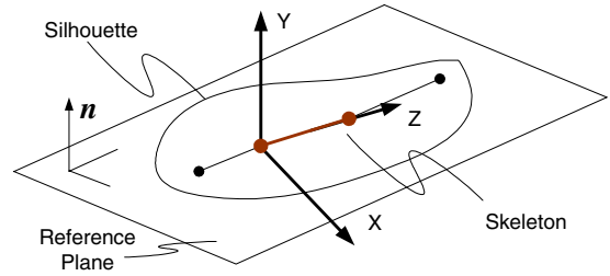
Figure 3: Local coordinate system of a line segment
