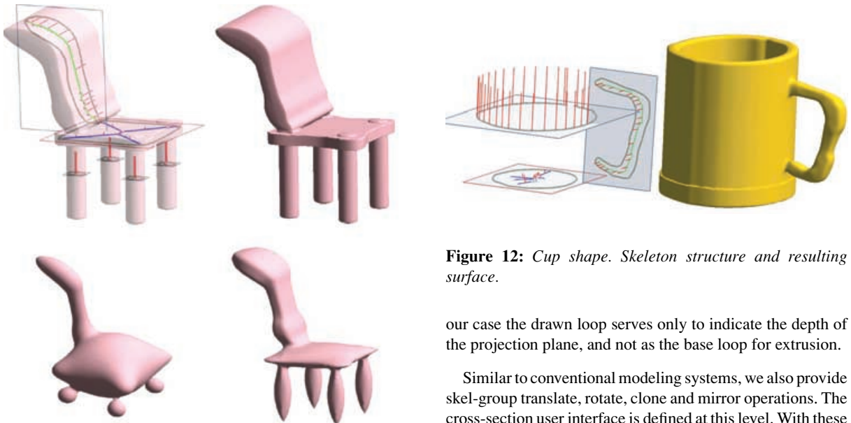
Figure 11: Chair shape. Skeleton structure (top left), generic surface (bottom left), rigid-style produced by our enhanced convolution model (top right), another style obtained by tuning the parameters of \mathcal{T} (bottom right).
