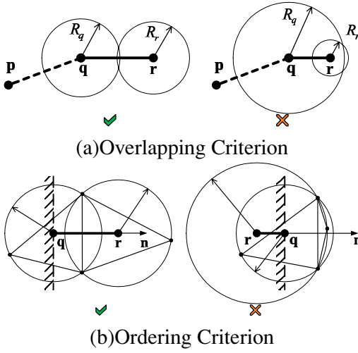
Figure 6: Skeleton filtering criteria.
