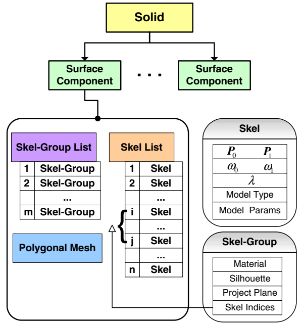
Figure 9: Data structure of our prototype design system.
