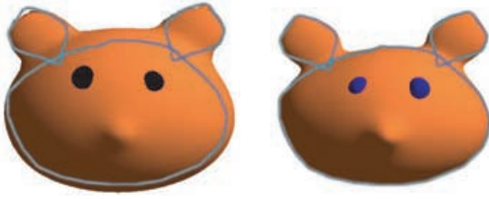
Figure 8: The resulting implicit surfaces without (left) and with (right) the global fitting step.
