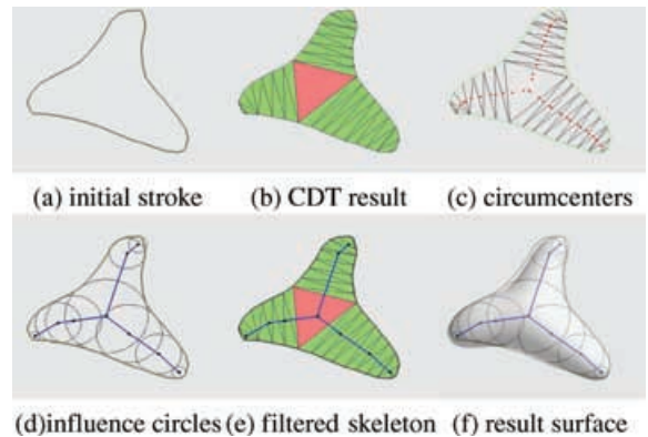
Figure 5: Generating convolution surface from silhouette
