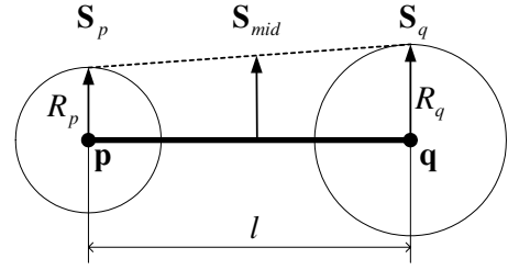
Figure 7: Convolution surface from a line segment.
