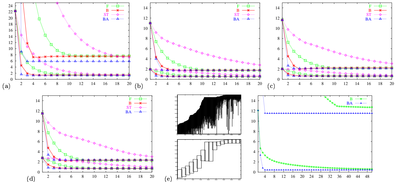
Figure 1: Experimental results: (a) synthetic data; (b) full Castle data; (c) alternate Castle data; (d) inner Castle data; (e) Wilshire data. The following symbols are used in all plots: F and B stand for the proposed F actorization and B ilinear algorithms, and ST and BA respectively stand for the S turm- T riggs and B undle A djustment techniques.
