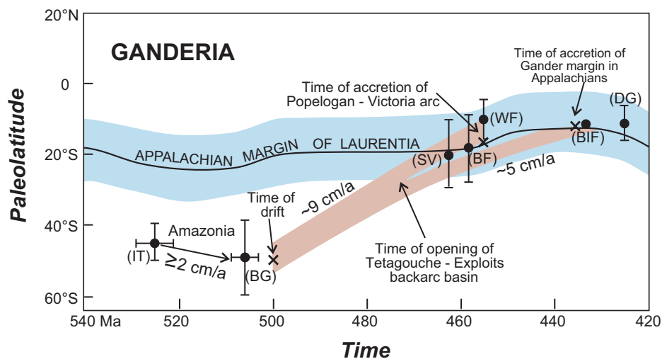
Figure 2. Early Paleozoic paleolatitudes and their errors (references in text) for Amazonia (IT—Itabaiana dikes) and Ganderian rocks in North America (BG—Bourinot Group; BF—Bluffer Pond Formation; BIF—Big Indian Pond Formation; WF—Winterville Formation; SV—Stacyville volcanics) and Ireland (DG—Dunquin Group), compared with predicted paleolatitudes of Appalachian margin of Laurentia (from MacNiocail, 2000, and references therein). Errors on predicted paleolatitudes are \sim 10^\circ . Errors of radiometric ages of rocks are indicated. Ages based on fossils have errors \leq 5 m.y.
