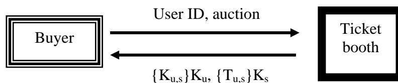
Figure 2 Ticket Granting Process
