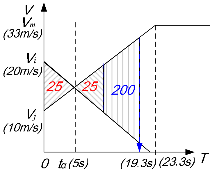
FIG. 59: An example scenario for simulation Case II. When v_i(0) = 20m/s , v_j(0) = 10m/s , a_i = -1m/s^2 and a_j = 1m/s^2 , the link duration is 19.3s. The numbers in the shaded areas are the distance values between the sender and the receiver.
