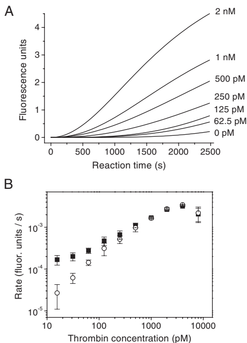
Figure 3. Characteristics of the thrombin-dependent proximity extension-mediated RCA reaction. (A) Real-time fluorescence traces of proximity extension-mediated RCA over a range of thrombin concentrations. (B) Dependence of maximal RCA rate upon thrombin concentration. Uncorrected rates for 16 pM–8 nM thrombin (black squares) and background-corrected rates (open circles). The background 0 pM thrombin rate is 1.04 \pm 2.3 \times 10^{-4} arbitrary fluorescence units per second.
