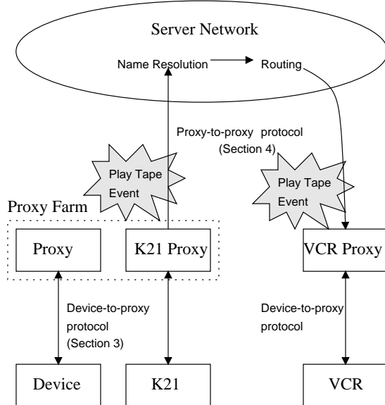
Figure 1: System Overview
