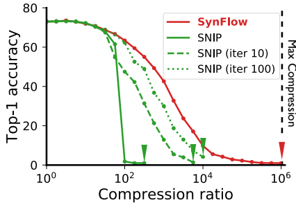
Figure 7: Iteration improves SNIP, but layer-collapse still occurs. Top-1 test accuracy as a function of the compression ratio for a VGG-16 model pruned at initialization and trained on CIFAR-100.
