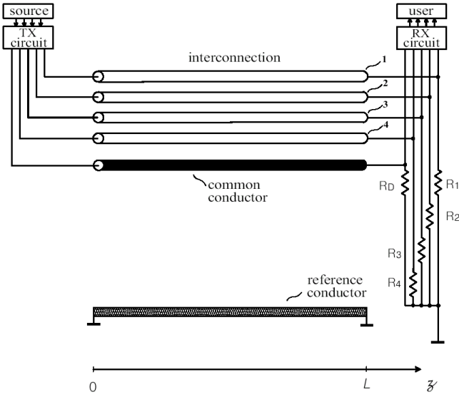
Fig. 2. A conventional PDL using a termination made of grounded resistors.
