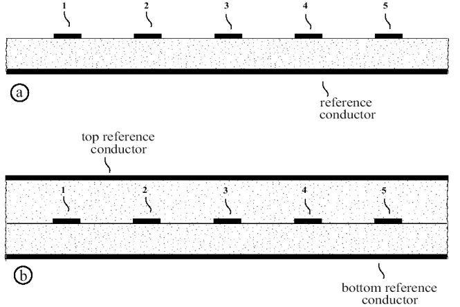
Fig. 3. Two possible cross-sections for the interconnection used in Fig. 2, where 1 to 4 are the TCs and 5 is the CC.
