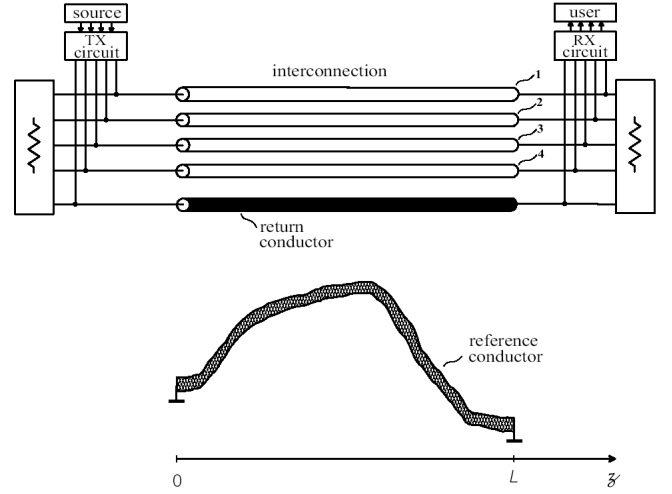
Fig. 5. A PDL implementing the ZXnoise method. At each end, the block containing the resistor symbol is a termination circuit. In some cases (e.g. unidirectional link), the termination circuit on the left is not present.
