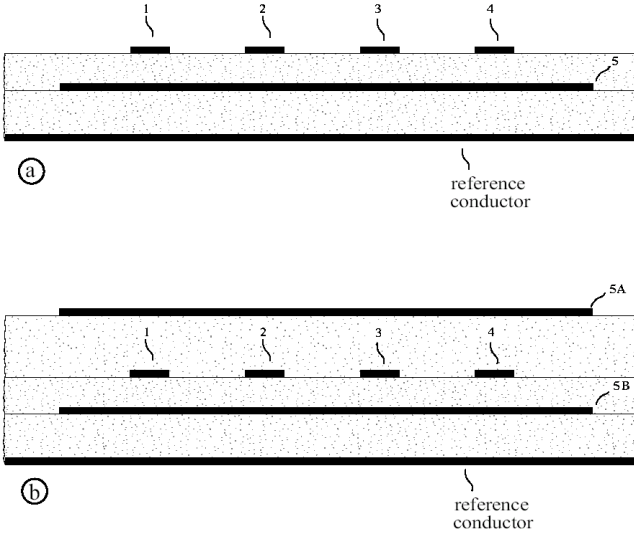
Fig. 4. Two possible cross-sections for the interconnection used in the ZXnoise method, where 1 to 4 are the TCs, where 5 is the RC in the coplanar-strips-over-return-conductor structure (a) and where the RC is made of the conductors 5A and 5B in the coplanar-strips-inside-return-conductor structure (b).
