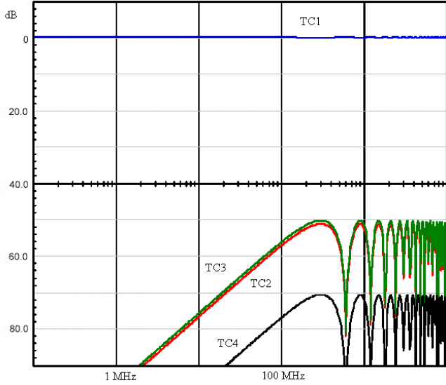
Fig. 6. Loss at the far-end for TC1 to TC4, when TC1 is excited at the near-end.
