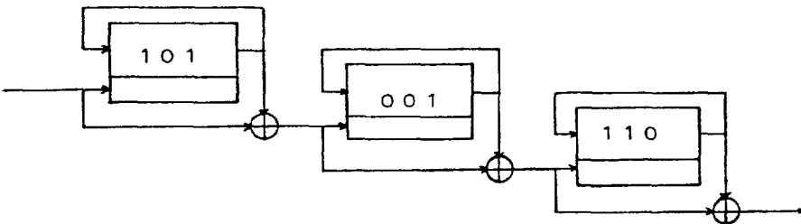
Fig.1. A cascade connection of clock controlled shift registers.
