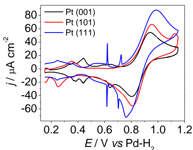
Figure 7. Cyclic voltammograms of 2 mM \text{FeSO}_4 in 10 mM \text{H}_2\text{SO}_4 on : Pt(111) electrode (blue line), Pt(001) electrode (black line) and Pt(101) electrode (red line) vs Pd-H 2 . Scan rate was 10 mV s -1 .
