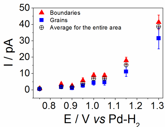
Figure 8. I - E curves for 1 mM \text{FeSO}_4 in 10 mM \text{H}_2\text{SO}_4 . The current was obtained by averaging the current from regions of the SECCM images where grain boundaries ( \blacktriangle ) and regions within the boundaries ( \blacksquare ) were identified. Similarly, an I - E curve for the average current over the entire scanned region (including all grains and boundaries) is also shown ( \oplus ) for comparison.
