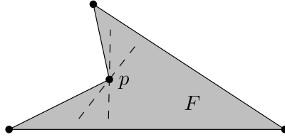
FIGURE 12. The lifting must be horizontal on every segment in F passing through p .
