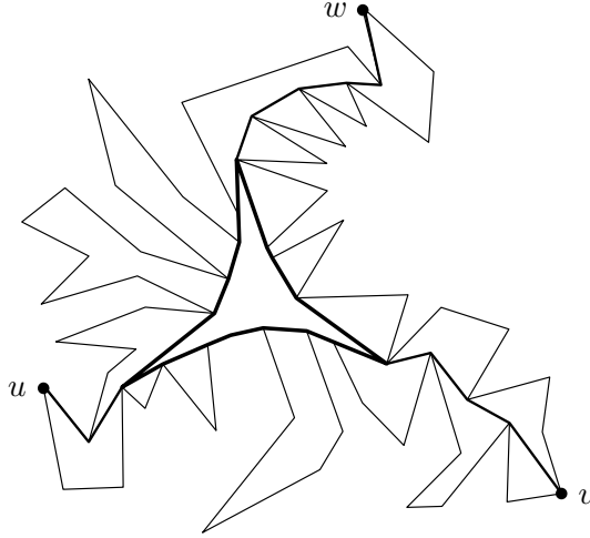
FIGURE 27. A geodesic triangle.
