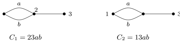
Figure 4. Admissible collections.
