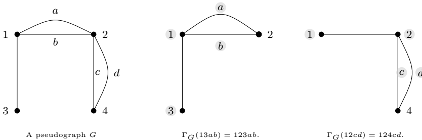
Figure 11. Examples of \Gamma_G .
