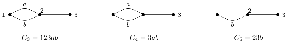
Figure 5. Non-admissible collections.
