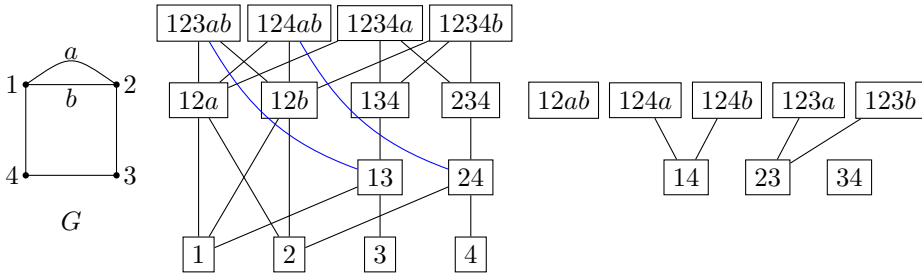
Figure 14. Neither S_{C,G}^{\text{odd}} nor S_{C,G}^{\text{even}} is shellable.
