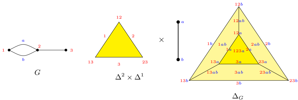
Figure 2. An example of \Delta_G whose facets are labelled with L_I .
