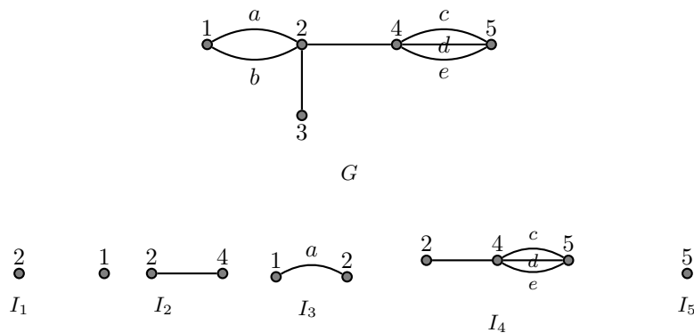
Figure 1. A pseudograph G and its subgraphs.
