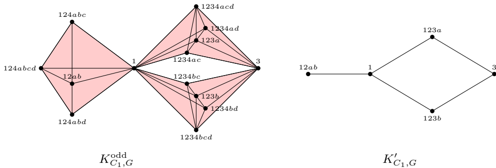
Figure 9. For the pseudograph G and C_1 = 13ab in Figure 8, two simplicial complexes K_{C_1, G}^{\text{odd}} and K'_{C_1, G} are homotopy equivalent.
