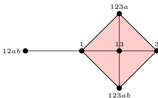
Figure 13. The order complex of S_{C_2,G}^{\text{odd}} for an admissible collection C_2 = 13ab .
