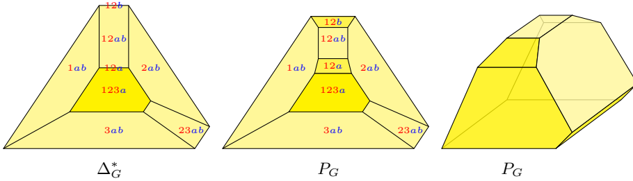
Figure 3. The pseudograph associahedron P_G .
