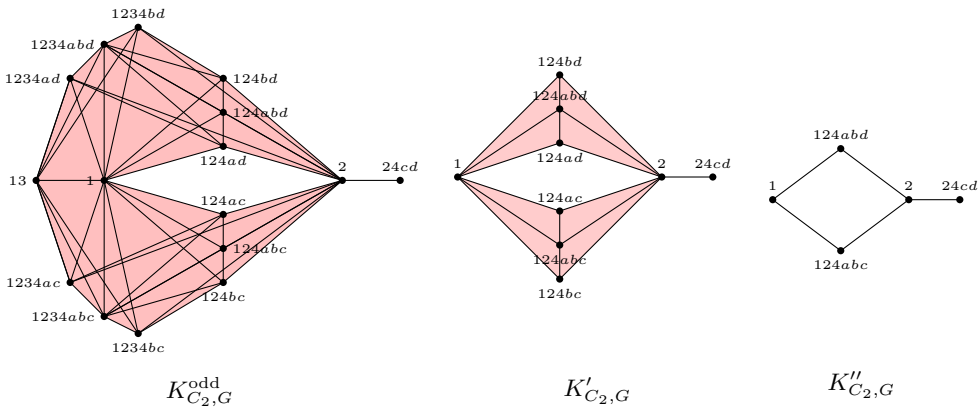
Figure 10. For C_2 = 12cd , three simplicial complexes K_{C_2,G}^{\text{odd}} , K'_{C_2,G} , and K''_{C_2,G} are homotopy equivalent.
