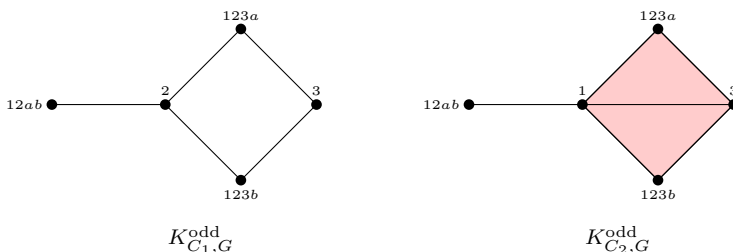
Figure 6. Simplicial complexes corresponding to admissible collections.
