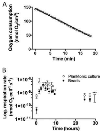
FIG 6 Respiration rate of P. aeruginosa PAO1. (A) Linear decrease in O 2 concentration over time exemplified by the respiration rate of alginate-encapsulated P. aeruginosa after 4 h 50 min growth ( r^2 = 0.998 ; P < 0.0001 ). (B) Volumetric respiration rates, R , for alginate-encapsulated and planktonic P. aeruginosa calculated from the change in O 2 concentrations at different time points during the experiment. Bars represent averages \pm standard errors of the means from three or four replicates. ***, P < 0.0001 .
