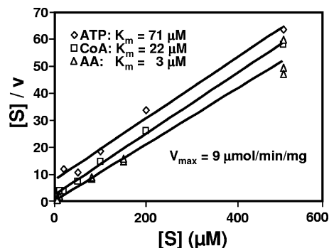
FIG. 5. Hanes plots for anthranilate, CoA, and ATP. Each substrate was varied independently in reaction mixes containing saturating amounts of the other two substrates. The substrate concentration ([S]) is plotted on the abscissa, and the reaction velocity ( v ; micromoles per minute per milligram of protein) is plotted on the ordinate. Values represent the average of results from three assays. K_m value estimates were determined from the x intercept ( x intercept = -K_m ), and V_{max} values were determined from the slope (slope = 1/V_{max} ) as described by Hanes (33).
