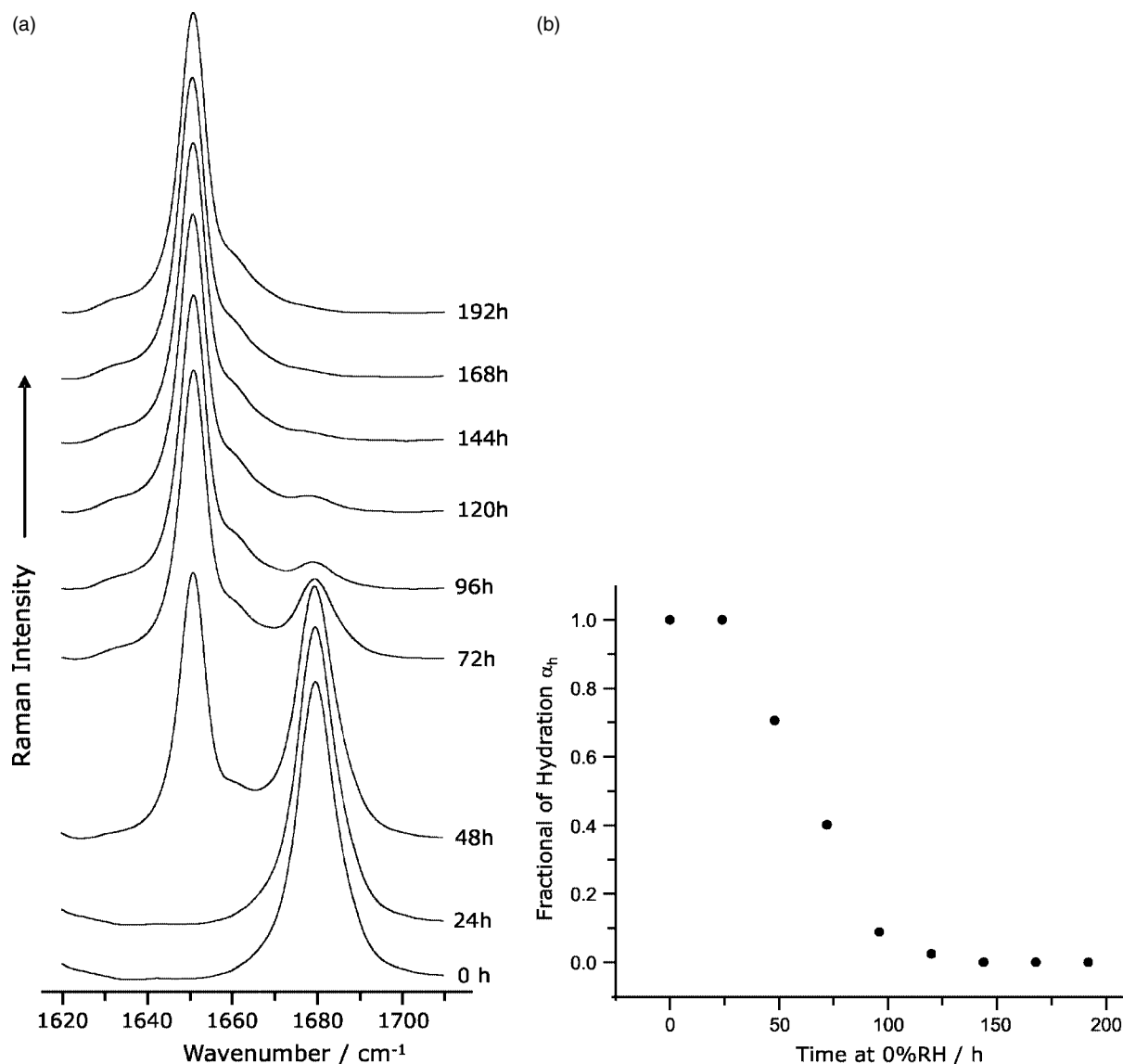
Figure 6. (a) Partial Raman spectra ( 1620\text{--}1710 \text{ cm}^{-1} ) of NCh samples stored at 0% RH ( 24^\circ\text{C} ) for up to 1 week; (b) plot of the measured \alpha_h ratio as a function of time-of-exposure to the 0% RH environment. Equivalent figures were also obtained for the 620\text{--}646 \text{ cm}^{-1} spectral region.
