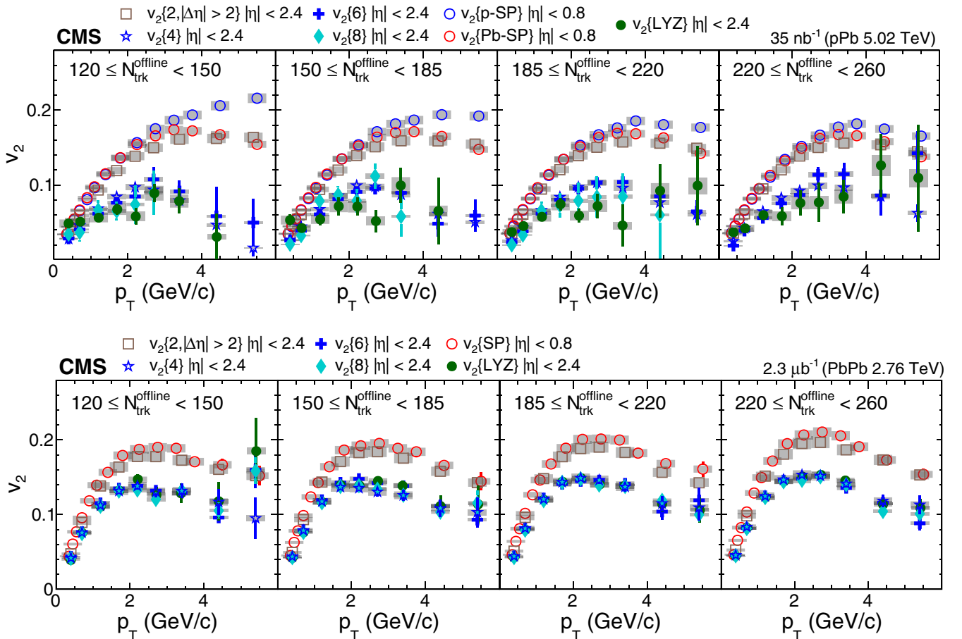
FIG. 1. (Top) The v_2 coefficients as a function of p_T in p Pb collisions for different N_{\text{trk}}^{\text{offline}} ranges. (Bottom) Same, but for PbPb collisions. The v_2\{2, |\Delta\eta| > 2\} and v_2\{4\} results are from Ref. [38]. For the p Pb collisions, the notations p -SP and Pb-SP indicate the pseudorapidity side of the reference event plane, and correspond to the p - and Pb-going directions, respectively. Pseudorapidities are given in the laboratory frame. Systematic uncertainties are indicated by the gray boxes.
