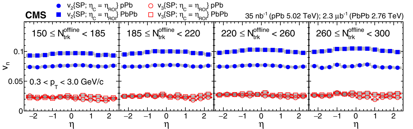
FIG. 11. The v_2 and v_3 values for p Pb (PbPb) collisions at \sqrt{s_{NN}} = 5.02(2.76) TeV with \eta_C = \eta_{ROI} . The v_n\{SP\} results are based on the furthest HF event plane in pseudorapidity. Pseudorapidities are given in the laboratory frame. Systematic uncertainties are indicated by the gray boxes.
