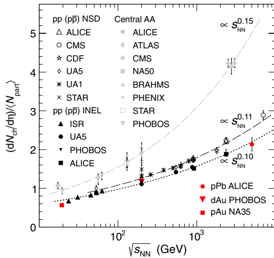
FIG. 2 (color online). Charged-particle pseudorapidity density at midrapidity normalized to the number of participants, calculated with the Glauber model, for p + \text{Pb} , p + \text{Au} , and d + \text{Au} [8,9] collisions as a function of \sqrt{s_{\text{NN}}} , compared to NSD [10–16] and inelastic [12,17–19] pp ( p\bar{p} ) collisions as well as central heavy-ion [19–30] collisions. The curves \propto s_{\text{NN}}^{0.11} and s_{\text{NN}}^{0.15} (from Ref. [28]) are superimposed on the NSD pp ( p\bar{p} ) and central heavy-ion data, respectively, while \propto s_{\text{NN}}^{0.10} (from Ref. [18]) is superimposed on the inelastic pp ( p\bar{p} ) data.
