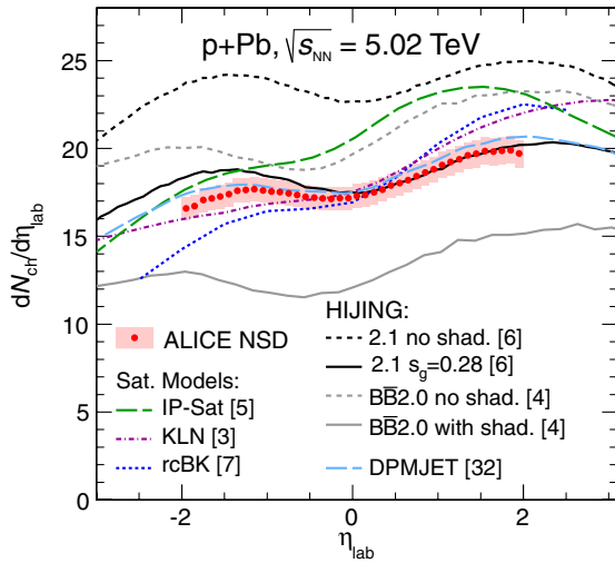
FIG. 1 (color online). Pseudorapidity density of charged particles measured in NSD p + \text{Pb} collisions at \sqrt{s_{NN}} = 5.02 TeV compared to theoretical predictions [3–7]. The calculations [4,5] have been shifted to the laboratory system.
