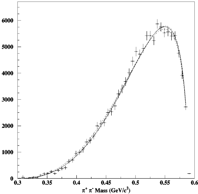
FIG. 6. Fits to the m_{\pi\pi} distribution. The points are the data corrected for efficiency, and the curves are the fit results. The smooth curve is the Novikov-Shifman model [Eq. (9)]. The long-dashed and short-dashed curves are the T. M. Yan model with and without higher-order corrections, and the dash-dot curve is the Voloshin-Zakharov model [Eq. (13)]. Three of the models are nearly indistinguishable. The T. M. Yan model without higher-order corrections is slightly different. The results are given in Tables V and VII.
