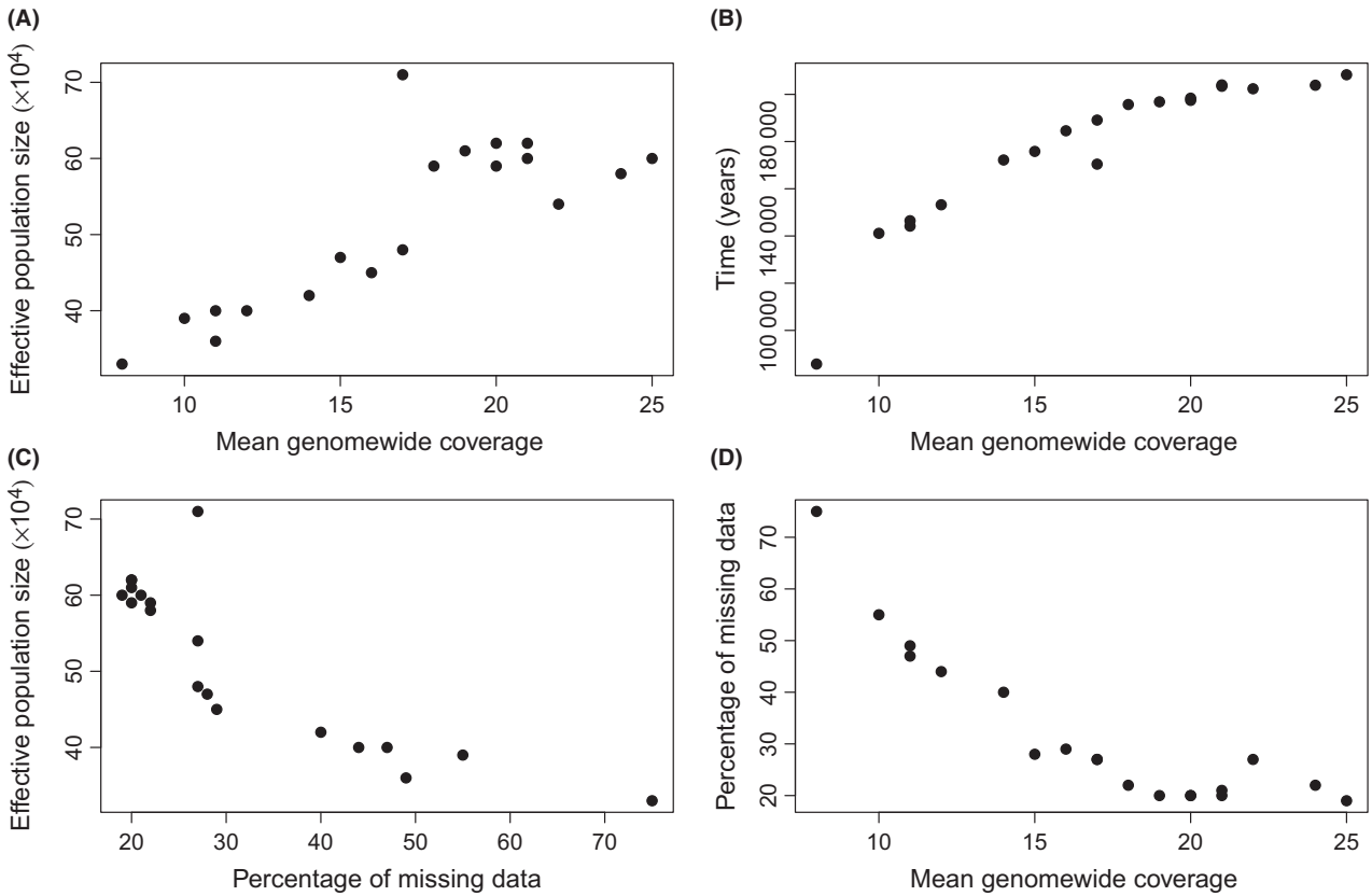
Fig. 4 Correlations between maximum N_e estimate and mean genomewide coverage (A), timing of the maximum N_e estimate and mean coverage (B), maximum N_e estimate and percentage of missing data (C), and percentage of missing data and mean coverage (D).
