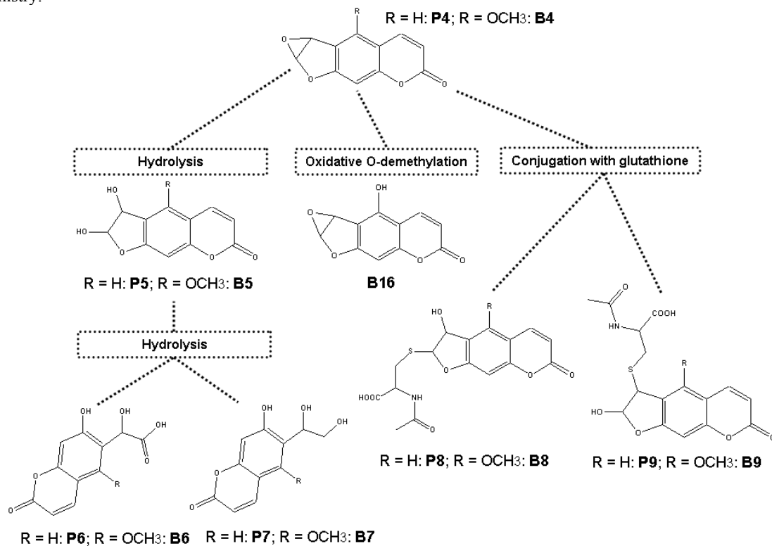
Figure 3. Metabolites and respective biotransformation reactions predicted for P1 and B1 using computational chemistry.
