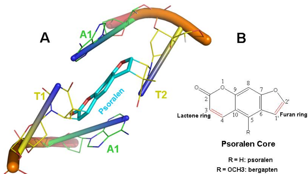
Figure 1. (A) Model for the cross-linkage between psoralen and thymine bases (T1 and T2). The psoralen molecule is intercalated between two pairs of the nucleotide bases adenine and thymine. (B) Chemical structure of psoralen core highlighting (in red) the sites in the furan and lactone ring which make covalent bonding with DNA molecule.
