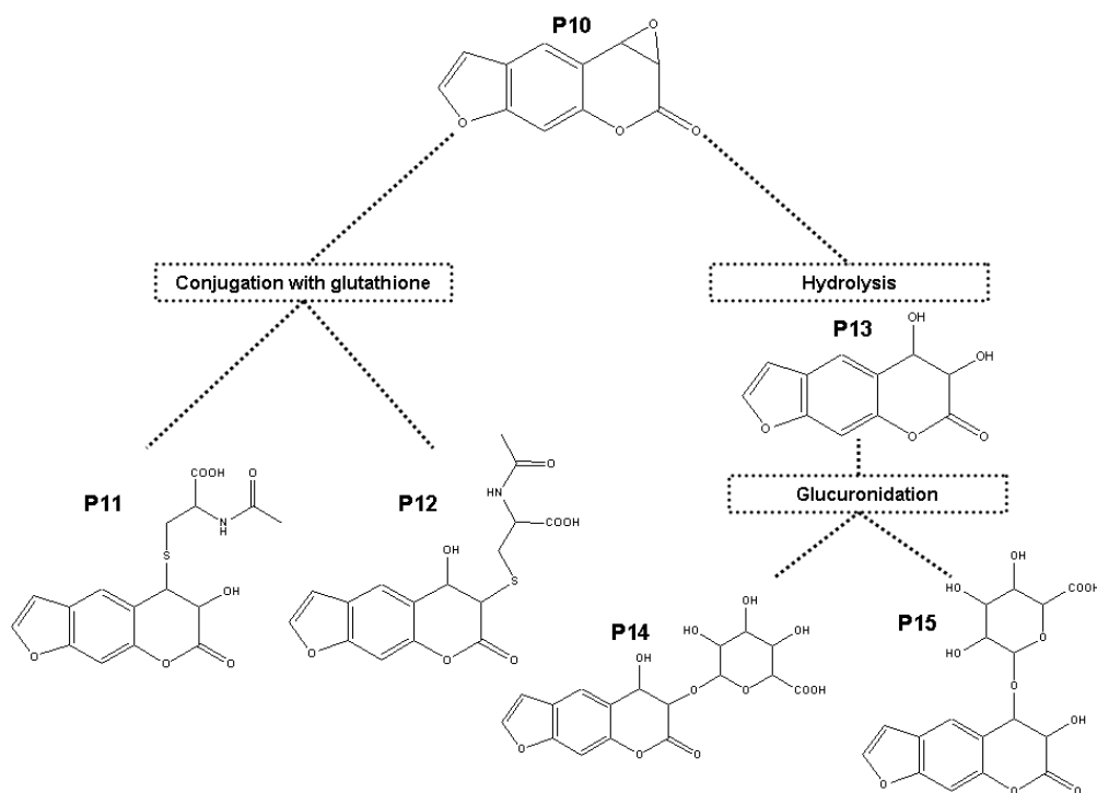
Figure 5. Metabolites and respective biotransformation reactions predicted for P10 using computational chemistry.
