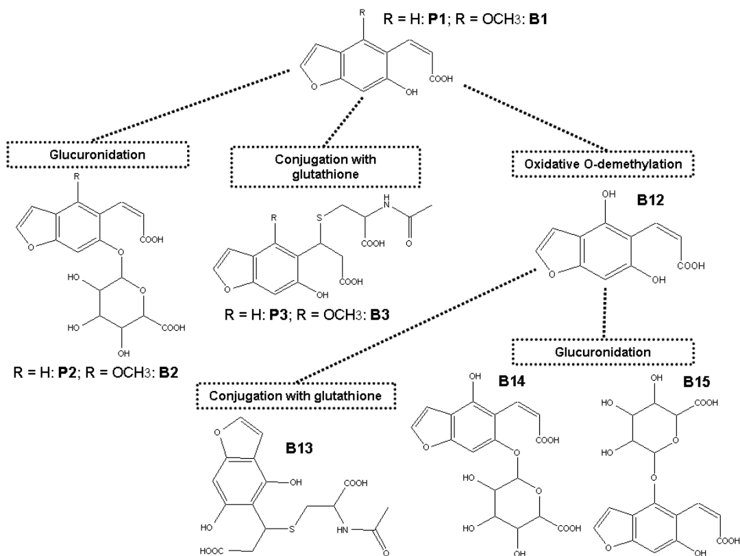
Figure 3. Metabolites and respective biotransformation reactions predicted for P1 and B1 using computational chemistry.
