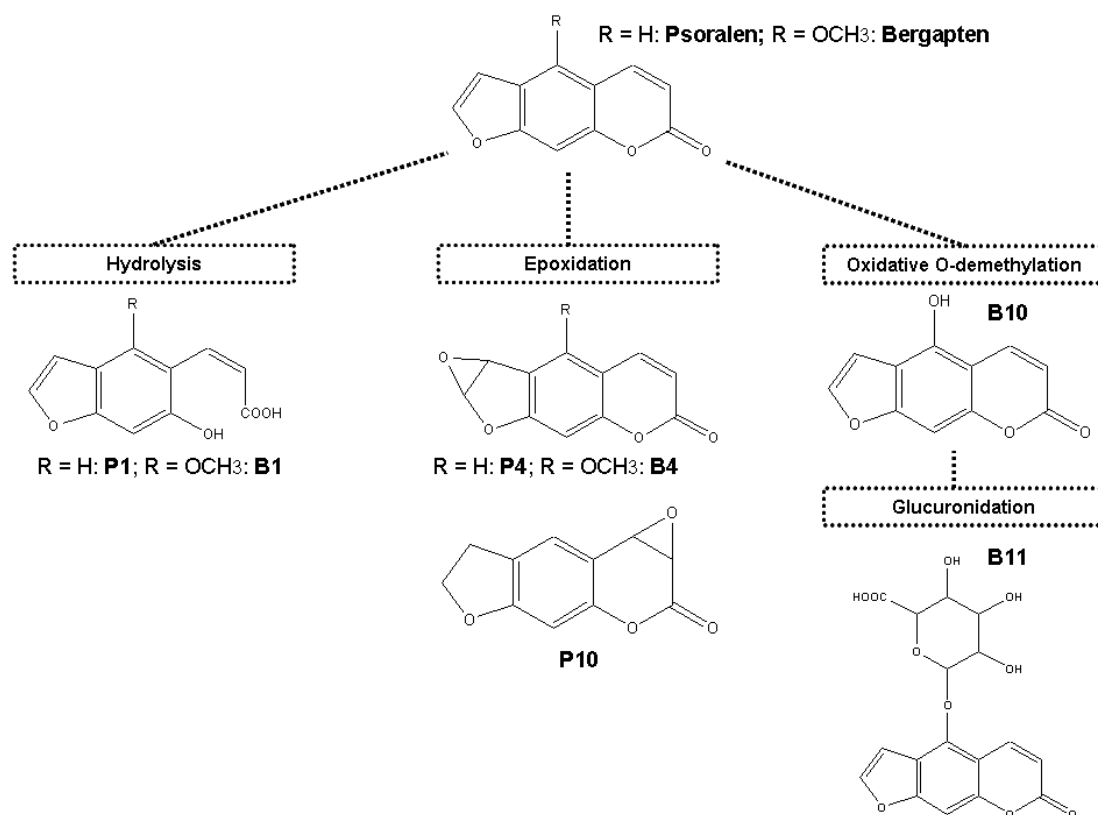
Figure 2. Metabolites and respective biotransformation reactions predicted for psoralen and bergapten using computational chemistry.
