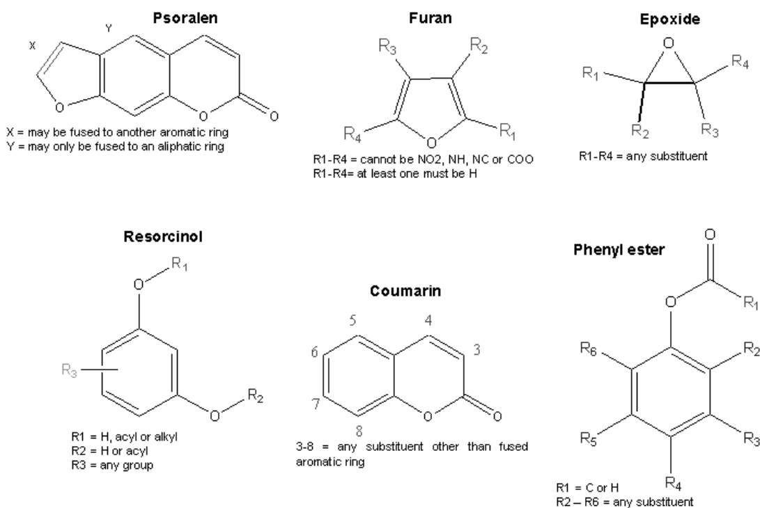
Figure 6. Chemical structures of six toxicophoric groups identified during computational chemistry analysis.
