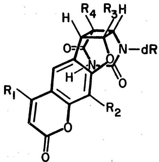
cis-syn-3
