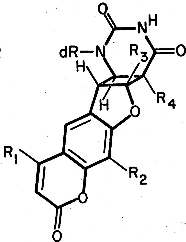
trans-anti-6
