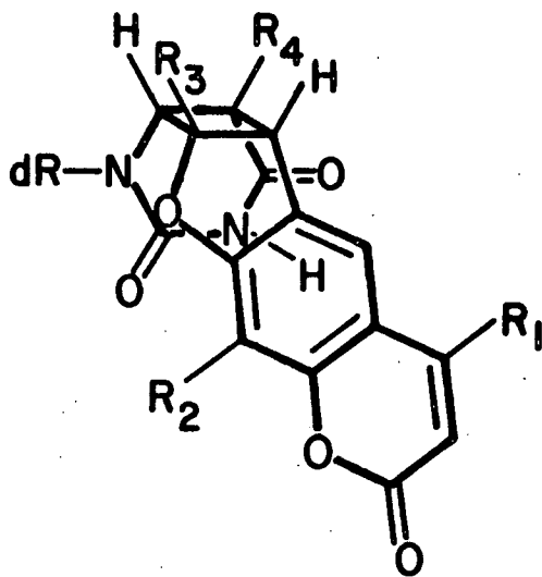
cis-syn-3'
