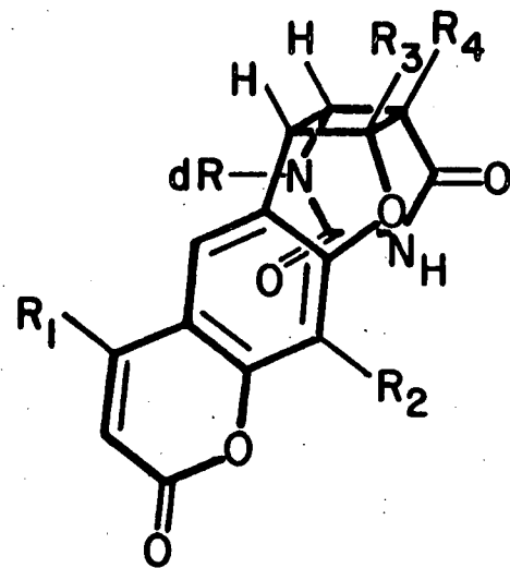
cis-syn-4
