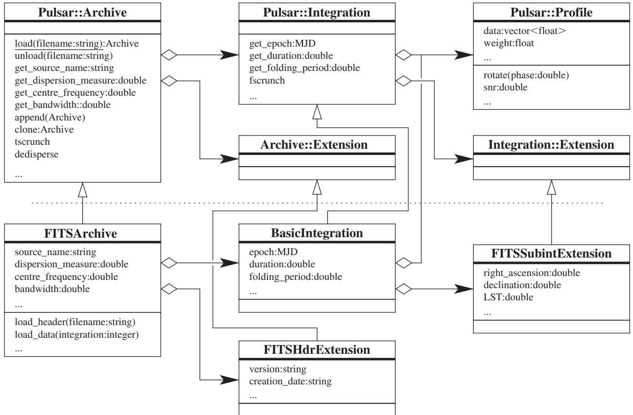
Figure 1 Class diagram of a portion of the PSRCHIVE library. The abstract base classes are shown above the dotted line. Below this line, the FITSArchive class implements Pulsar::Archive attribute storage and access methods, as well as methods for loading and unloading data to and from a PSRFITS file. The combined use of composition and inheritance enables complex structures and behaviours to be constructed using modular components.
