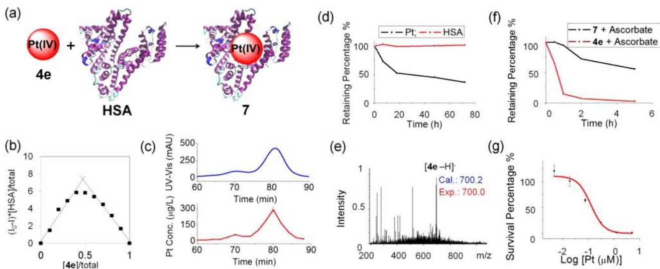
Figure 3. Systematic investigation of the Pt-HSA complex, 7: (a) schematic representation of the formation of 7; (b) Job plot of the Pt-HSA complex showing 1:1 stoichiometry; (c) FPLC trace of 7 and the corresponding GFAAS trace indicate that 4e is tightly bound to HSA; (d) dialysis experiment indicating that around 60% of the platinum compound was released from 7 over 72 h and that the HSA is retained within the 3 kDa MWCO micro-dialysis bag; (e) ESI-mass spectrum of the octanol extract showing an intense signal at m/z = 700.1 for [4e - H]^- supporting the integrity of 4e in 7; (f) octanol extraction analysis showing that >90% of 4e (3 \mu M) was reduced by ascorbate (30 \mu M) after 2 h incubation at 37 ^{\circ} C in the absence of HSA. The reduction was decreased to <50% by forming the Pt-HSA complex (3 \mu M); (g) cytotoxicity profile of 7 against A2780 human ovarian cancer cells showing an IC_{50} value of 0.12 \pm 0.01 \mu M.
