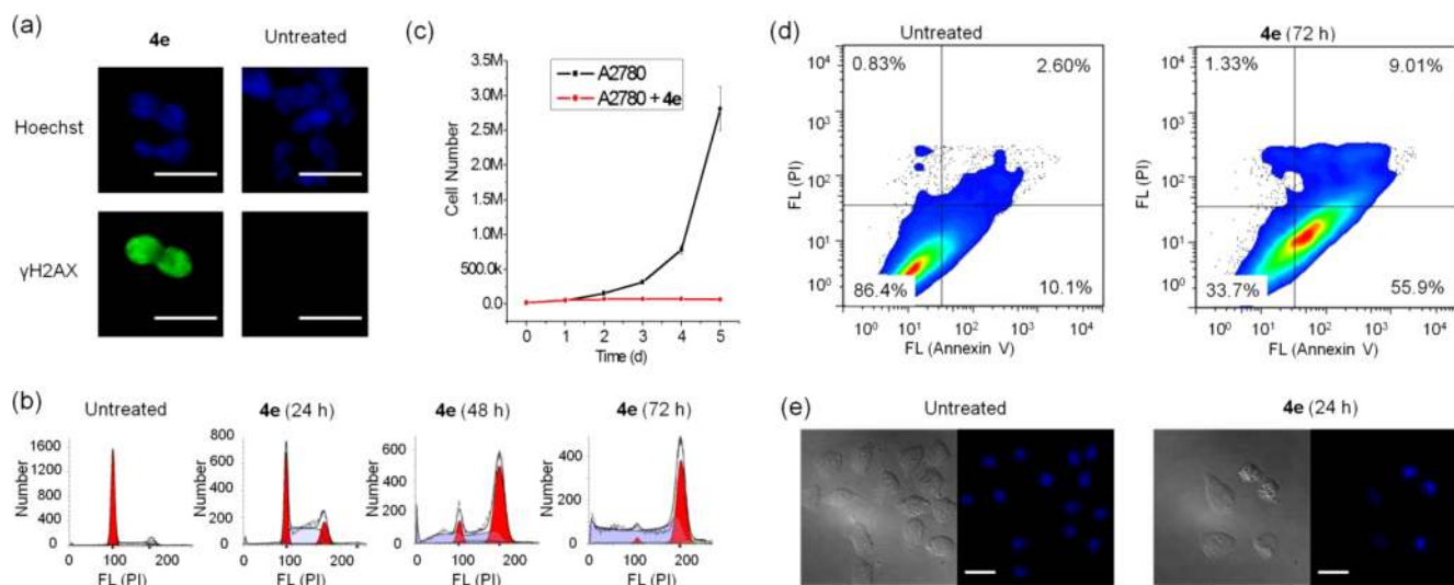
Figure 2. DNA damage and cellular responses of A2780 cells treated with 4e: (a) immunostaining of the biomarker of DNA damage, phosphorylated H2AX ( \gamma H2AX) (scale bar, 20 \mu m); (b) flow cytometric analysis of cell cycle indicating that 4e induced cell cycle arrest at the G2/M phase at 0.2 \mu M; (c) 4e can inhibit proliferation in A2780 cells at 0.2 \mu M; (d) Annexin V/PI coupled flow cytometric analysis showing 4e induced apoptosis in a large population of cells at 0.2 \mu M; (e) cellular images show characteristic apoptotic cell changes (blebbing, chromatin condensation, and nuclear fragmentation) upon treatment with 1 \mu M of 4e for 24 h (scale bar, 20 \mu m).
