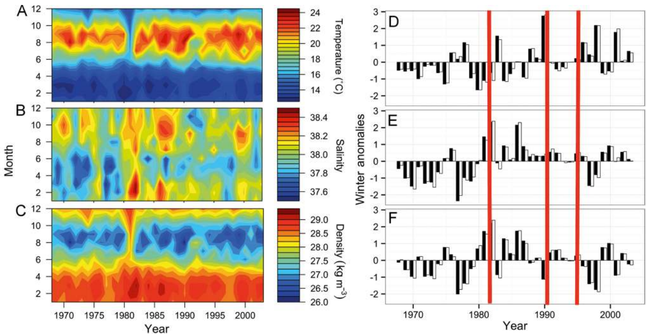
Fig. 4. Seasonal and inter-annual variability of (A) temperature, (B) salinity and (C) density at 20 m depth, and standardized winter (Jan–Mar) anomalies of (D) temperature, (E) salinity and (F) density at 20 (white bars) and 50 (black bars) m depths. Red lines: turning points in abundance of the zooplankton time series
