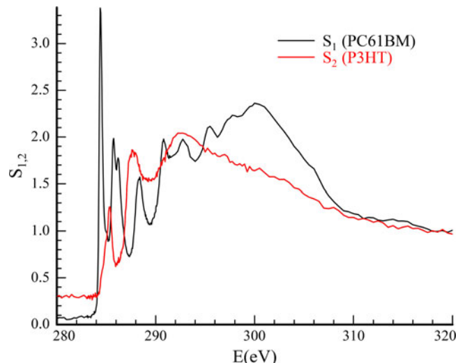
Fig. 1. Assumed reference spectra used in modeling of PC 61 BM (black) and P3HT (red), normalized to make intensities at 320 eV equal 1.
