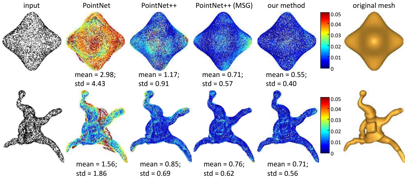
Figure 4. Visual comparison on samples from our collected dataset (top row) and SHREC (bottom row). The colors on points (see color map) reveal the surface distance errors, where blue indicates low error and red indicates high error.
