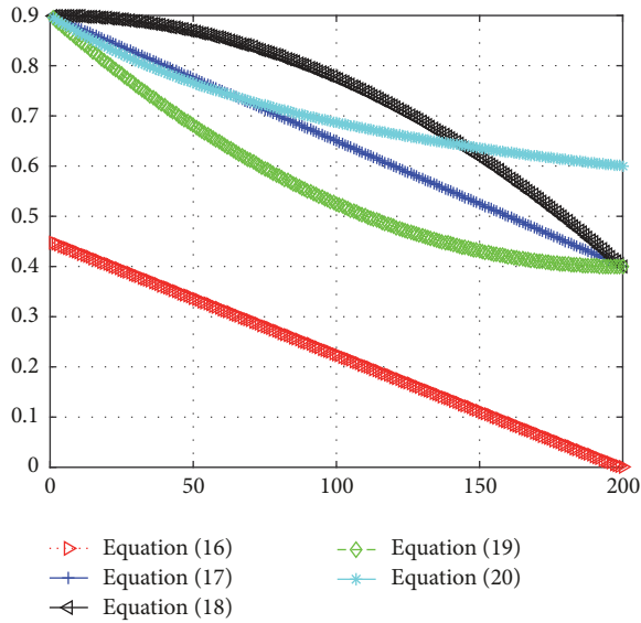
FIGURE 6: The variation curves of several dynamic inertia weights.
