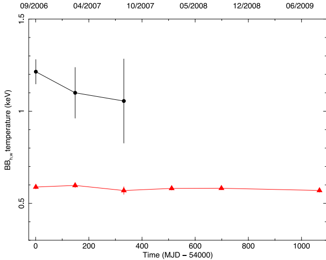
Figure 9. Temperature evolution of the BB used for modelling the peaks spectra. Black circles correspond to the hard component, red triangles to the warm component. The zero-point in time represents the onset of the 2006 outburst.
