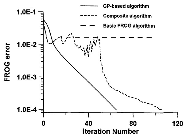
Fig. 2. Error in the retrieved FROG traces as a function of iteration number for the basic FROG algorithm, the composite algorithm, and the new GP-based algorithm for the double pulse. Whereas the basic FROG algorithm stagnates, the GP-based algorithm successfully retrieves this pulse. The composite algorithm also retrieves the pulse, but it is much slower (for iteration numbers larger than 50 the composite algorithm used the minimization method, a much slower method in real time than the basic or the GP-based algorithm).
