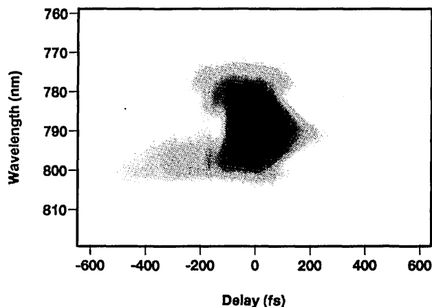
Fig. 3. Polarization-gate FROG trace of an amplified Ti:sapphire laser pulse.
