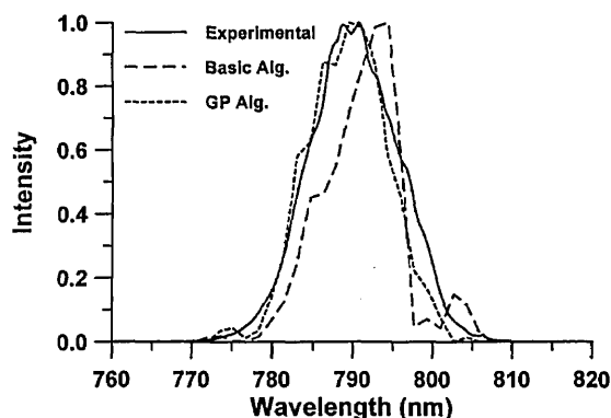
Fig. 4. Spectra retrieved by the basic FROG algorithm (long-dashed curve) and the GP-based algorithm (short-dashed curve) from the trace of Fig. 3 compared with the experimentally measured spectrum (solid curve). Clearly the GP-based algorithm gives better agreement with the experimental spectrum. The final rms error between the experimental and reconstructed traces was 0.0134 for the basic FROG algorithm and 0.00801 for the GP-based algorithm.
