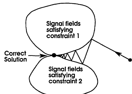
Fig. 1. Schematic of the method of generalized projections. The figure is pedagogical; in FROG the sets (which reside in a higher-dimensional space) may be of a more complicated structure.
