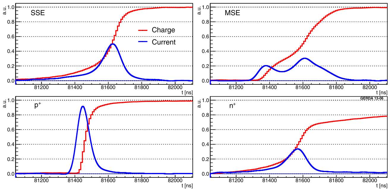
Fig. 2 Candidate pulse traces taken from BEGe data for a SSE ( top left ), MSE ( top right ), p+ electrode event ( bottom left ) and n+ surface event ( bottom right ). The maximal charge pulse amplitudes are
