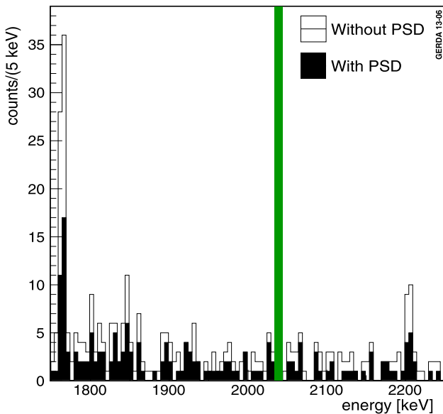
Fig. 21 Energy spectrum of semi-coaxial detectors with and without neural network PSD selection
