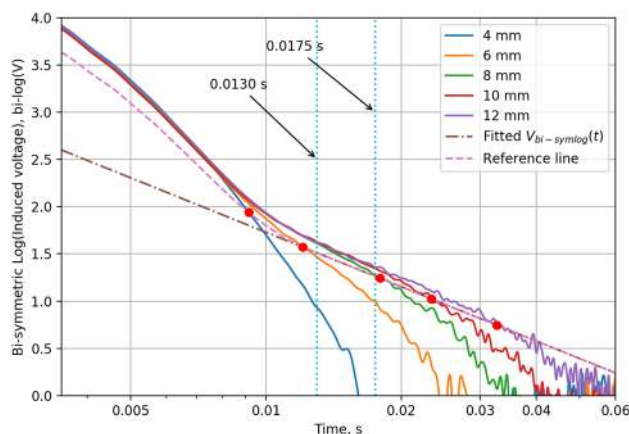
Fig. 4 Visualisation of reference line and PEC signals
