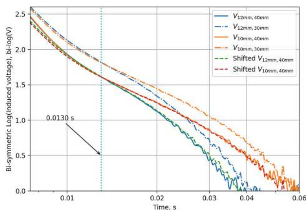
Fig. 5 Visualisation of normalised and non-normalised signals
