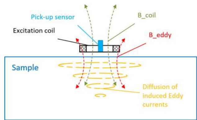
Fig. 2 Illustration of the working principle of ECT
