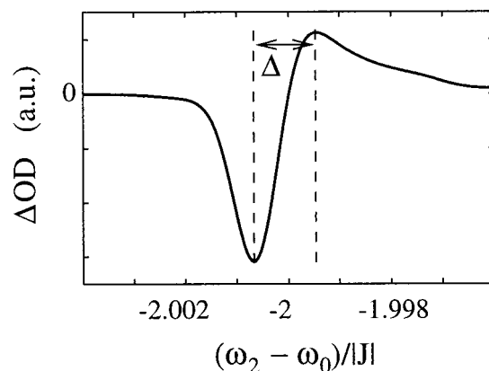
Figure 1. Typical pump–probe spectrum for a J aggregate as a function of the probe frequency \omega_2 . The spectrum shows a negative contribution due to bleaching and stimulated emission of one-exciton states excited by the pump laser, and a blue-shifted positive feature due to induced absorption from the excited one-exciton to two-exciton states. The spectral separation \Delta between both features is thought to be a measure of the exciton delocalization length, a conjecture that is tested in this paper. The spectrum shown here is a two-color pump–probe spectrum simulated for aggregates of 250 molecules with static disorder of strength \sigma/|J| = 0.01 (see section III). The pump frequency \omega_1 was taken at the maximum of the absorption band.
