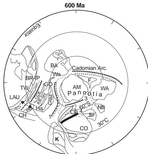
Fig. 8 Late Vendian (ca. 600 Ma) palaeogeographic reconstruction. Northern South America (AM) positions modified from Torsvik et al. (1996); Baltica based on McKerron et al. (1992); West Africa and Nigeria-Borborena (NB) as in Unrug (1996); Laurentia as in Torsvik et al. (1996); Congo and Kalahari craton positions based on data suggesting that the Damara orogen was intracratonic and the Rio de la Plata-Congo collided prior to the collision of the Kalahari vs Congo (see Prave 1996). F Florida Block; CH Chilena terrane; RR-SH Roanoke Rapids and Spring Hope belt; CCK Charlotte-Carolina-Kioke belt. Wa West Avalonia; CABA Cuyania-Antofalla-Belen-Arequipa terrane; 1 Puncoviscana-Tucavaca magmatic arc; 3 Paraguay-Araguay magmatic arc
